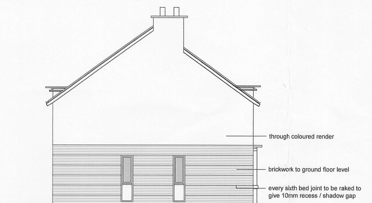
PROPOSED SIDE ELEVATION (UNITS 8 - 13 & 19)
