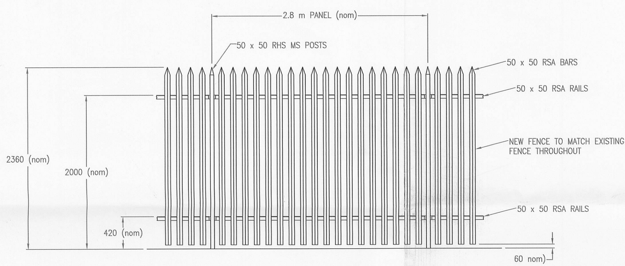
TYPICAL SECTION OF FENCE GALVANISED
