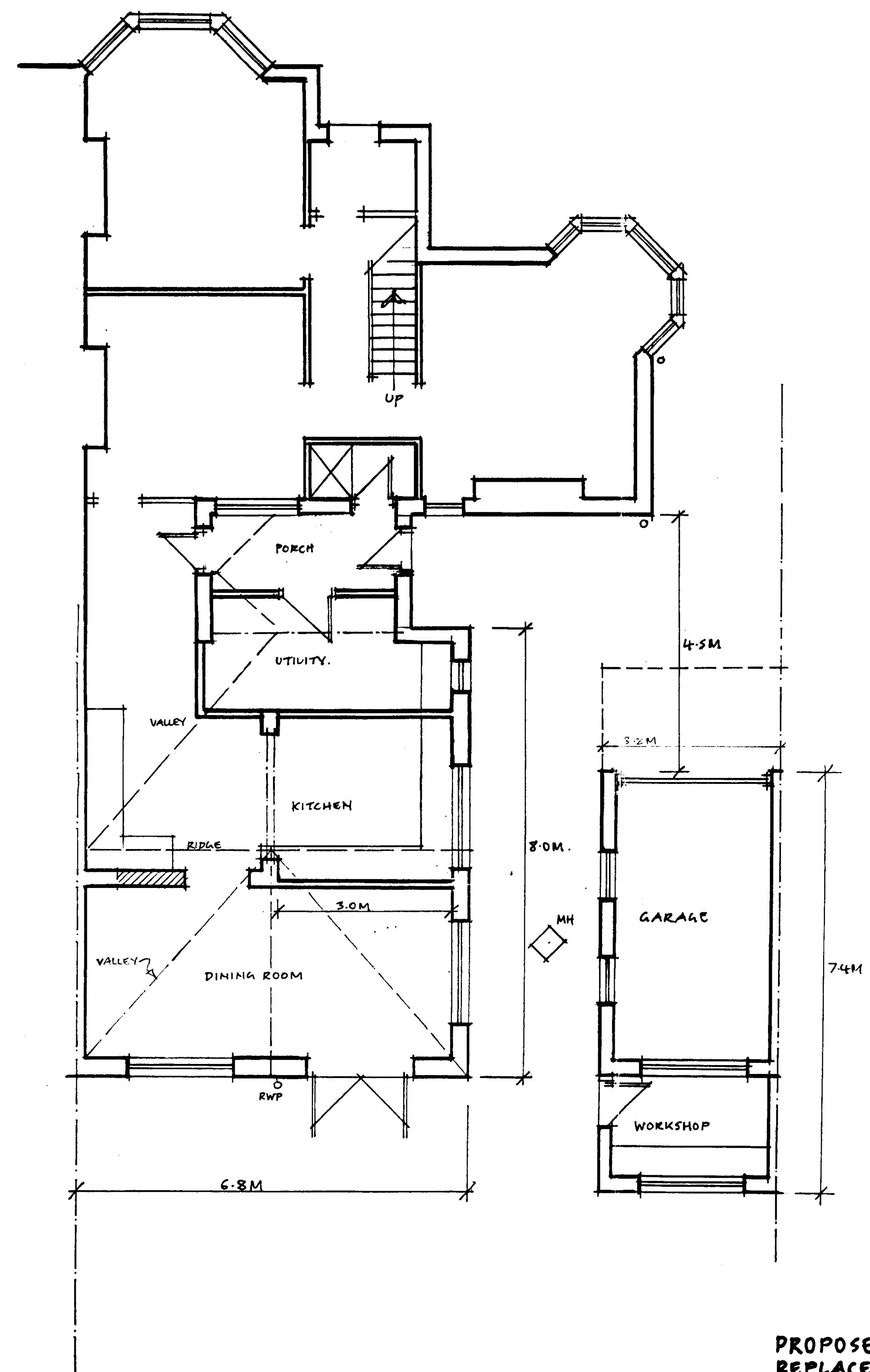
PROPOSED GROUND FLOOR PLAN 1:50
