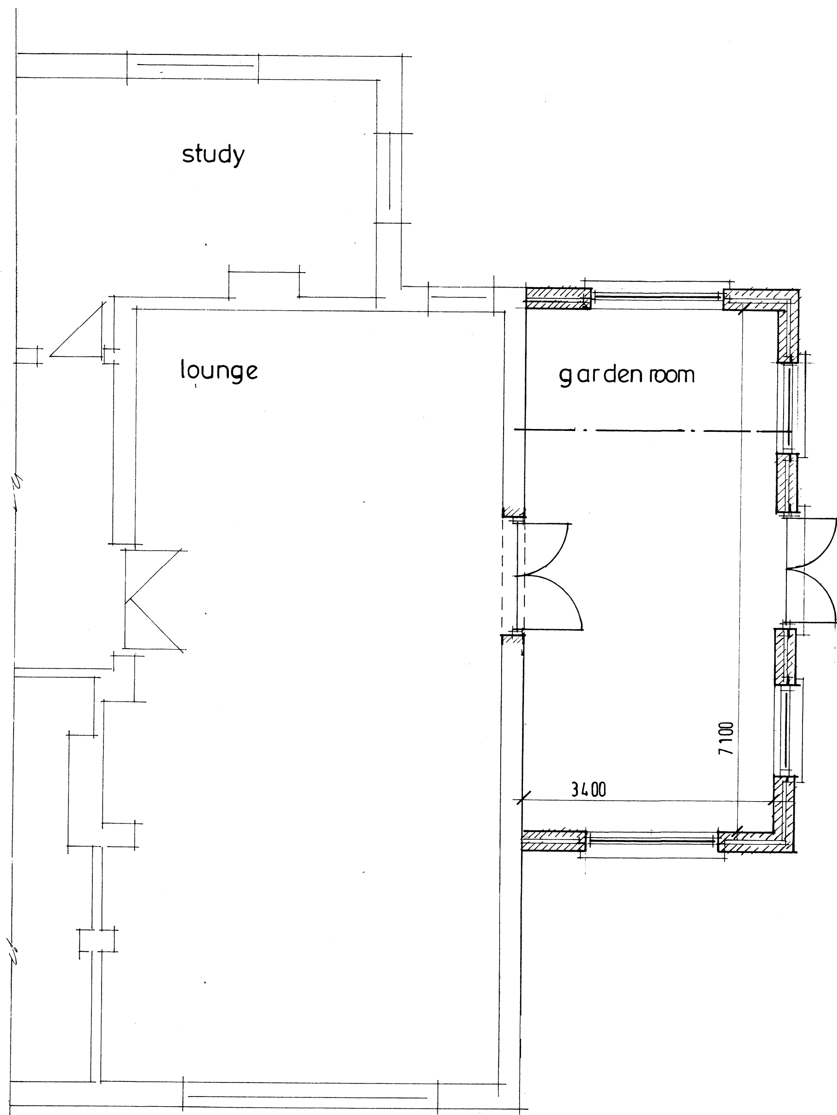
PART GROUND FLOOR
