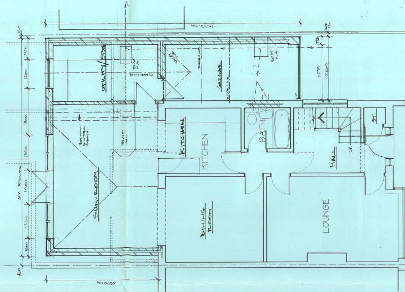
PROPOSED GROUND FLOOR PLAN 1:50
