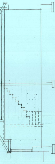
TYPICAL SECTION (SHEDDING LOFT CONVERSION) 1:50
