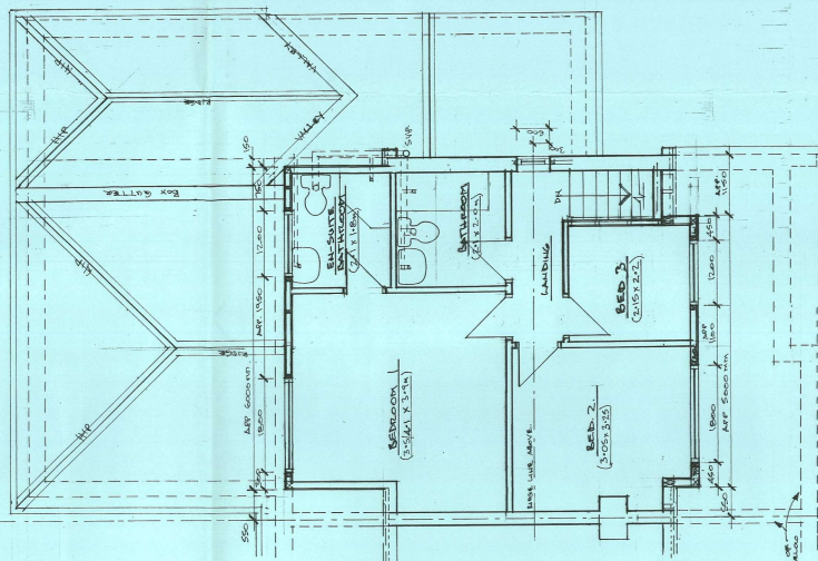
PROPOSED FIRST FLOOR PLAN 1:50
