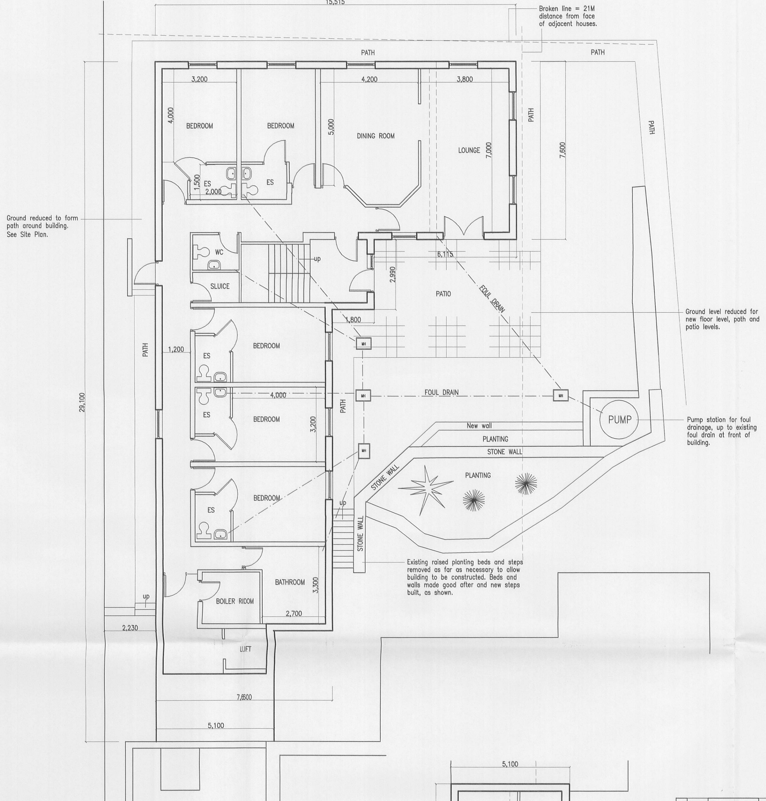
GROUND FLOOR PLAN OF EXTENSION
