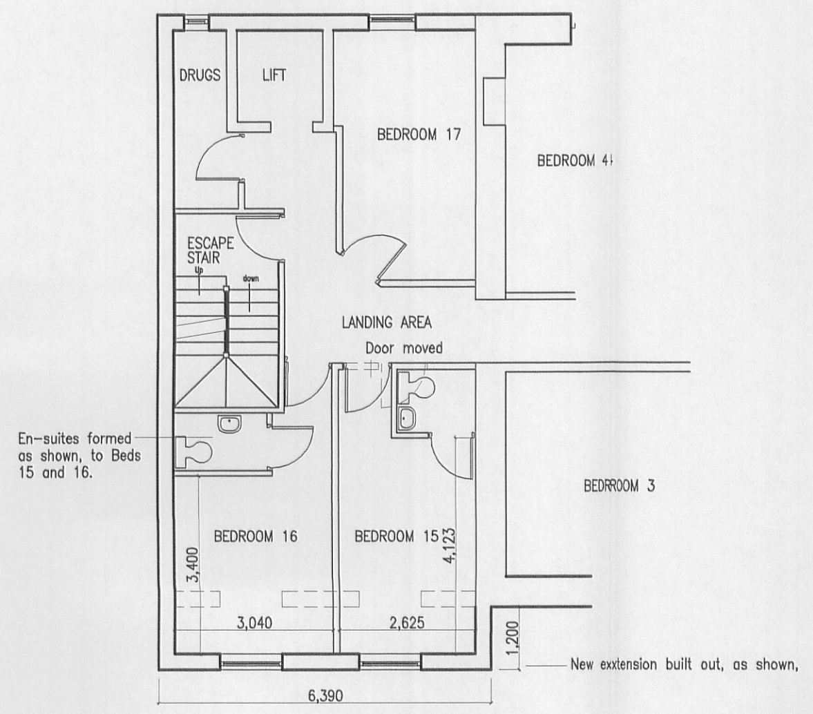
FIRST FLOOR PLAN EXISTING BUILDING
