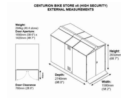
METAL SHED FOR 6no CYCLES BEING 2740mm DEEP AND 1580mm WIDE, WITH A HEIGHT OF 2030mm, POLICE APPROVED. SECURE WITH PADLOCK TO AMIN OF SOLD SECURE SILVER STANDARD. ALSO WITHIN UNIT PROVIDE 3no SHEFFIELD RACKS SECURED TO A SOLID FOUNDATION.
