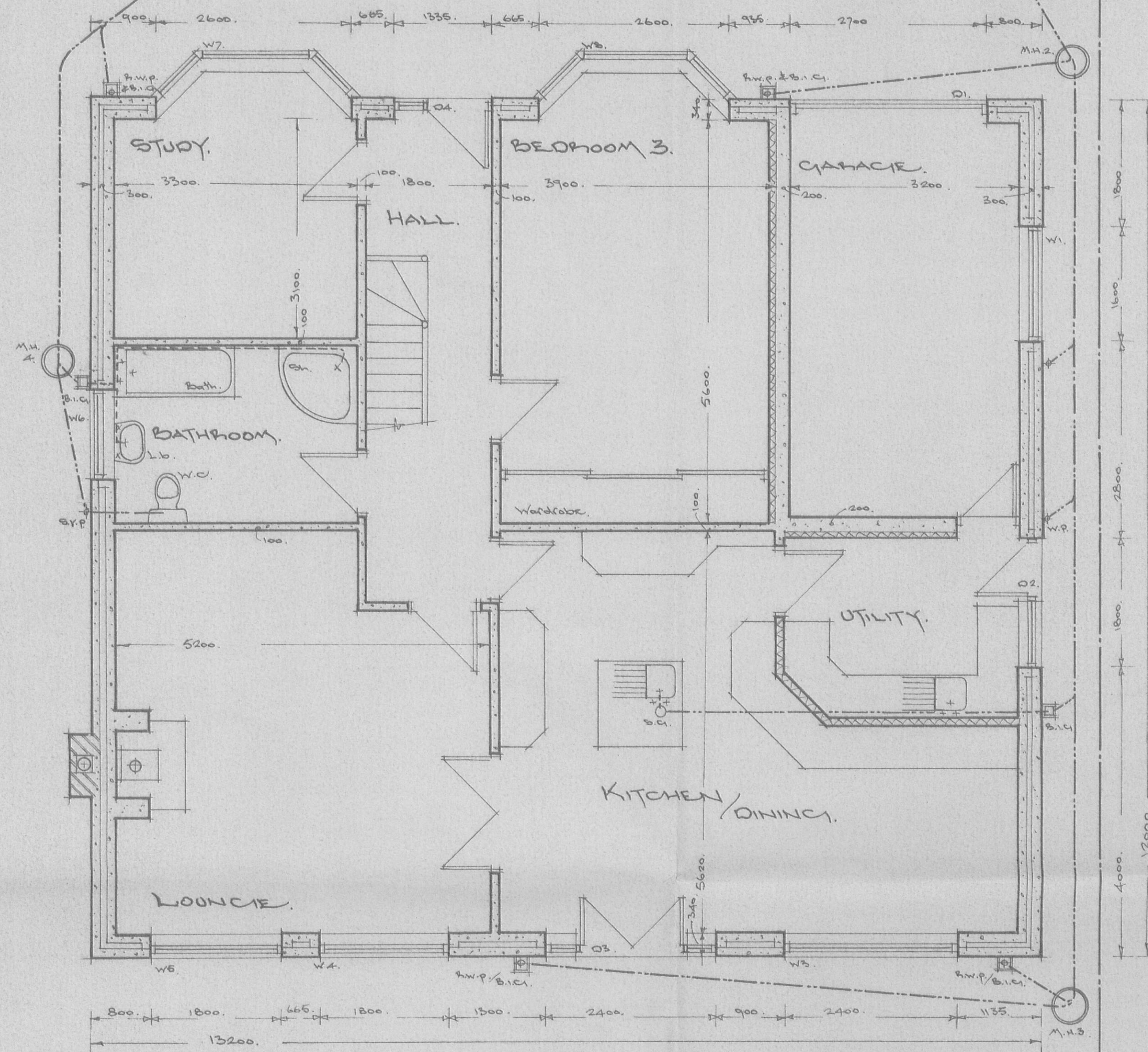
Ground floor plan. Scale: 1 to 50.
