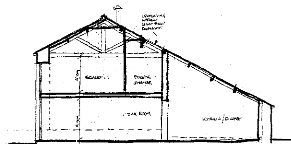
SECTION THRO' AA
