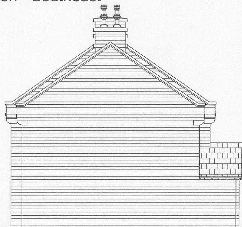
Rear elevation - Southeast
