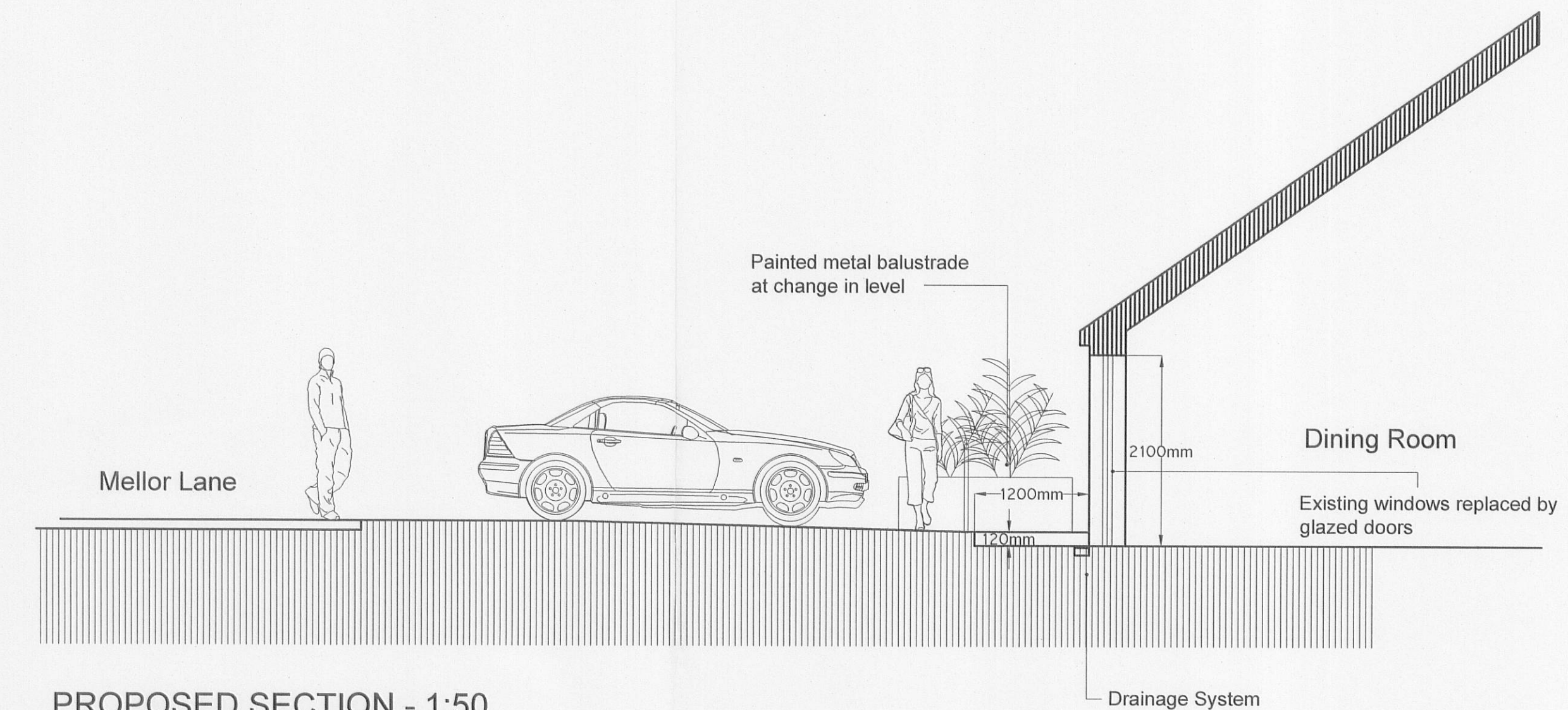
PROPOSED SECTION - 1:50
