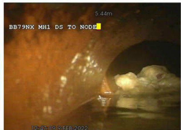
3-1-4A, 00:00:24, 5.44 m Collapsed drain or sewer, 75% area loss, REQUIRES EXCAVATION AND REPAIR
