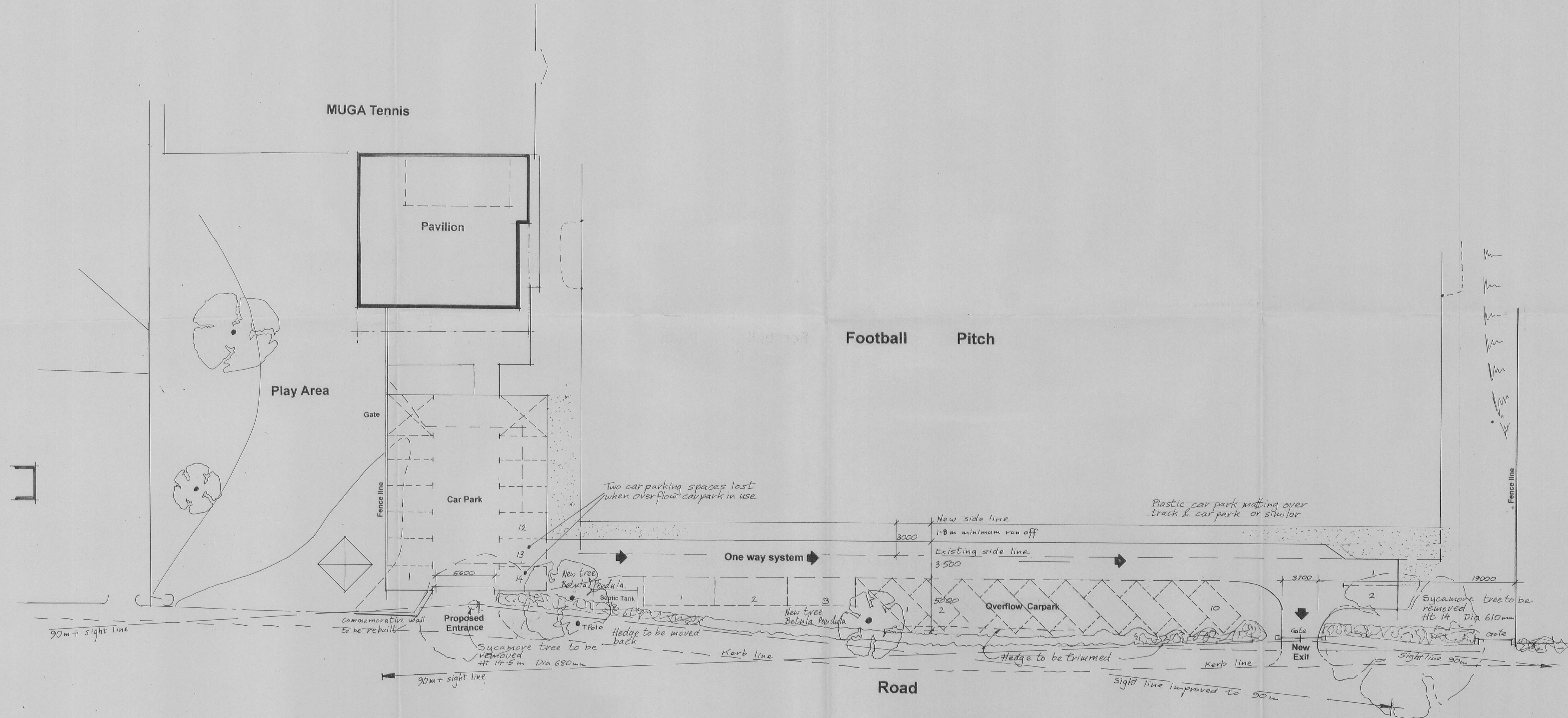
Site Layout
