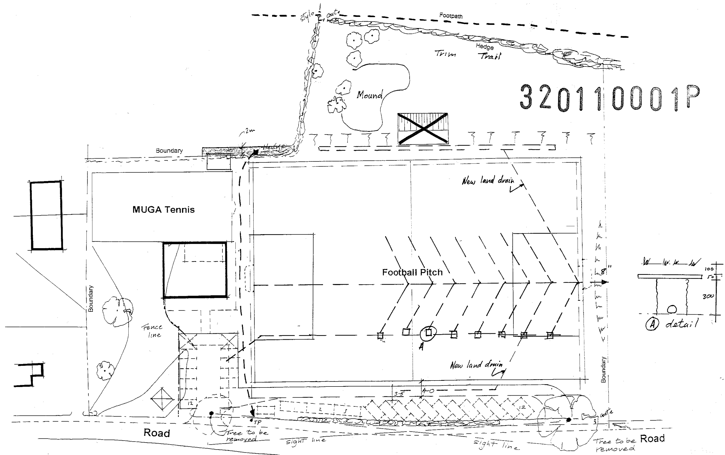
Site Layout
