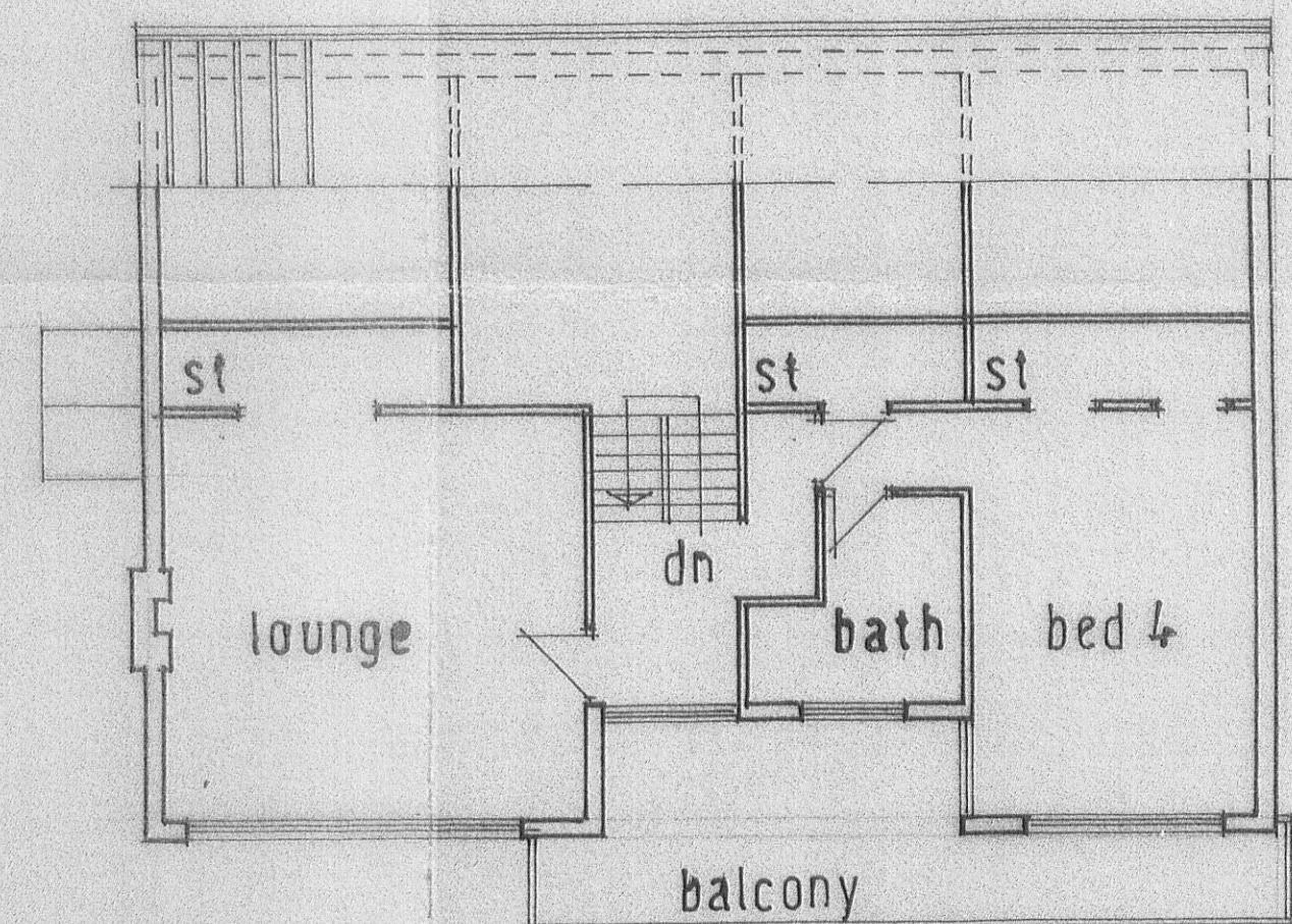
no 23 existing upper floor plan
