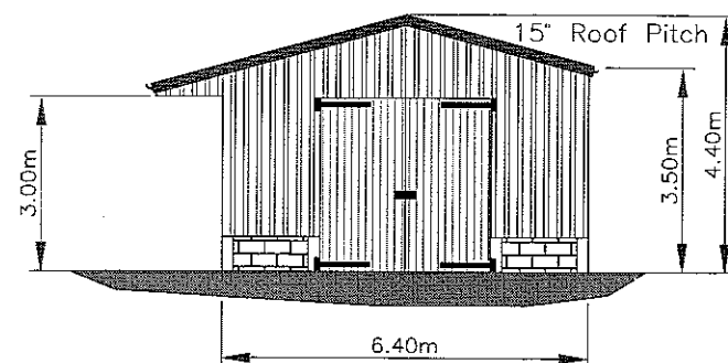
WEST FACING ELEVATION
