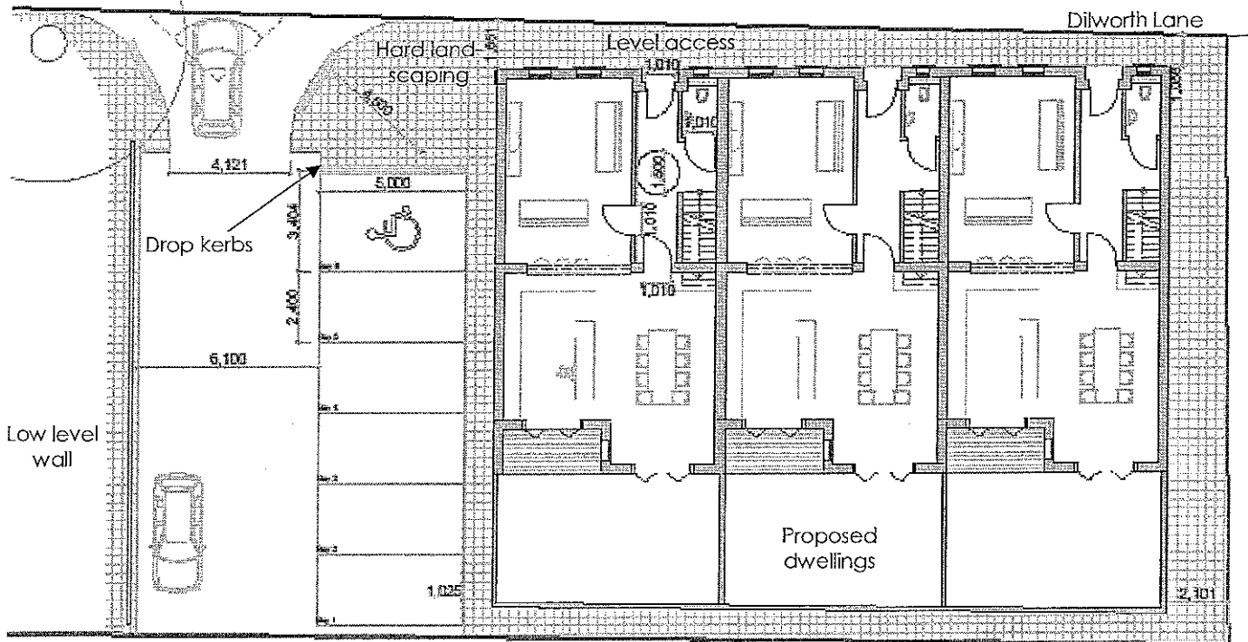
Fig 30. Parking arrangement
