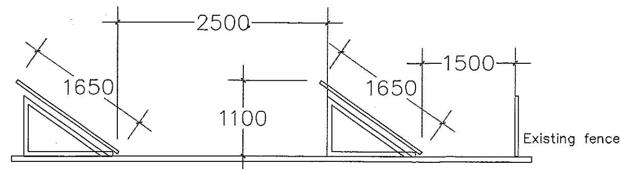
PROPOSED SECTION
