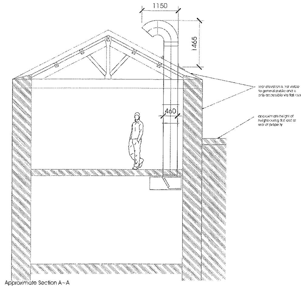
Approximate Section A-A
