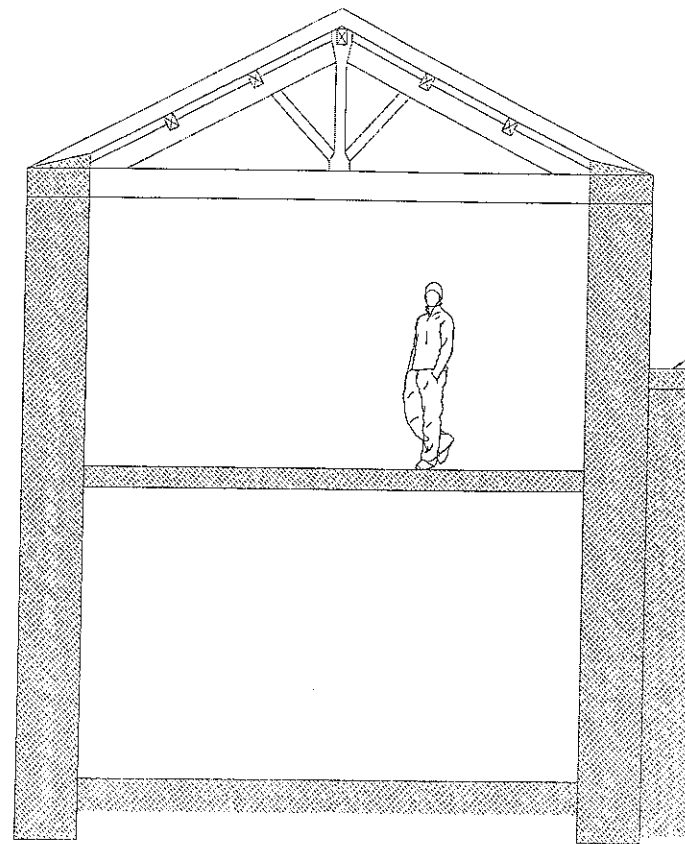
Approximate Section A-A
