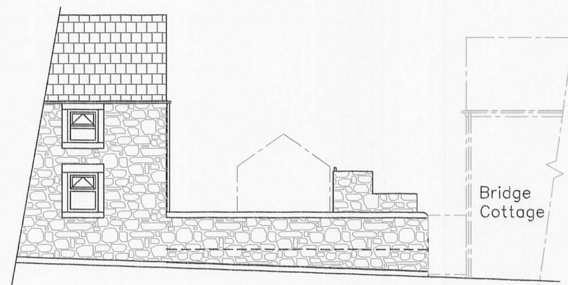
Existing South Facing Elevation
