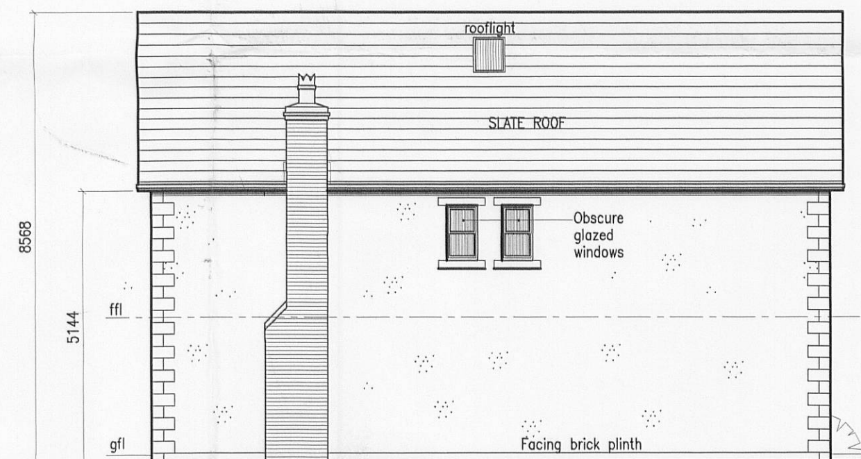
ELEVATION TO SUNNYMEADE COTTAGE
