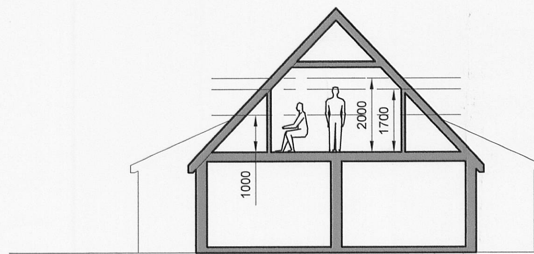
SECTION
