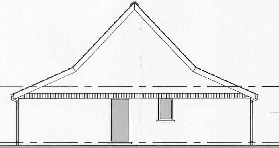
NORTH
