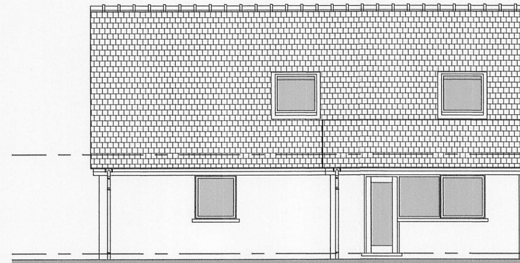
EAST
