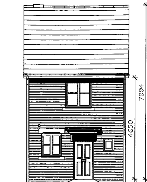
FRONT ELEVATION
