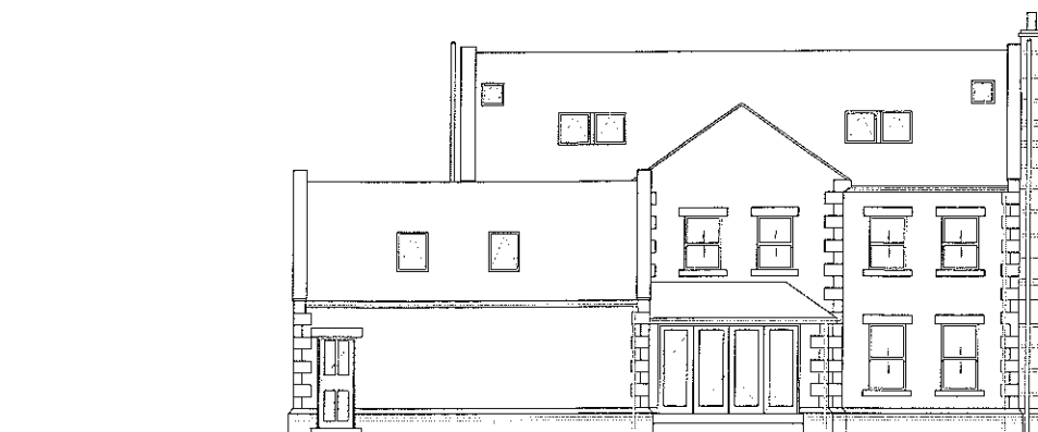
Rear Elevation
