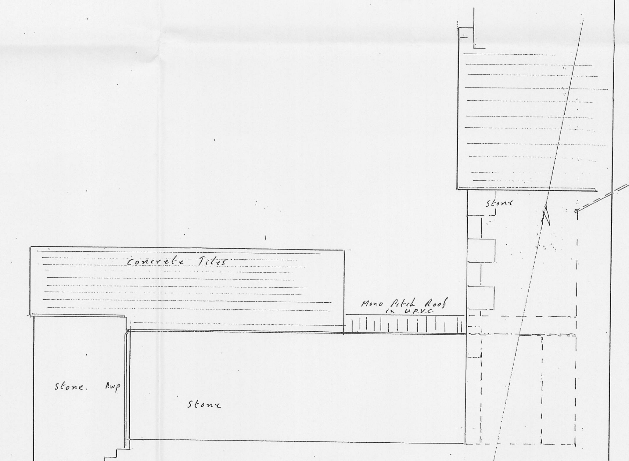
Eastern Elevation. (Part)
