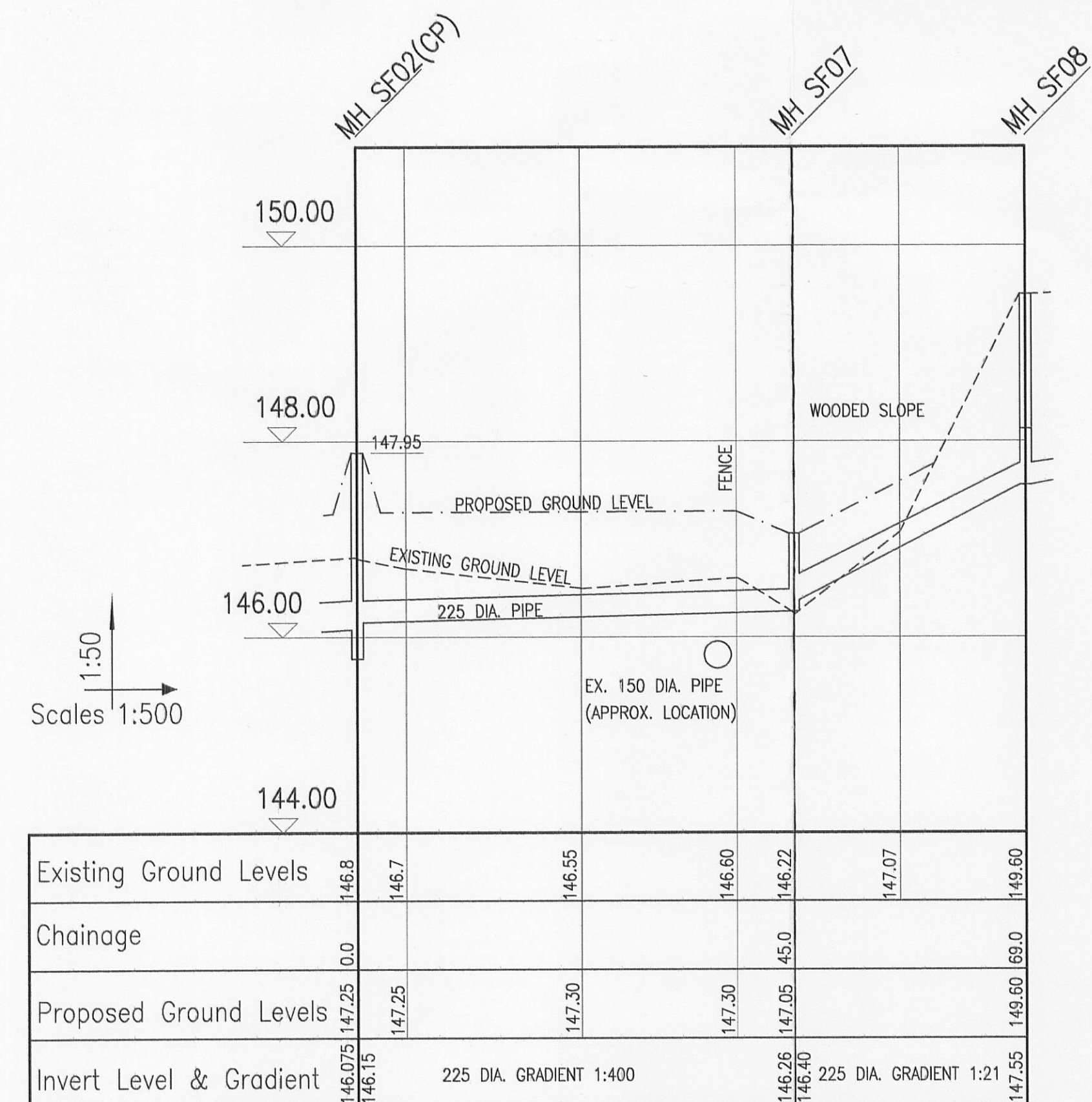
LONGITUDINAL SECTION MH SF02 TO MH SF08
