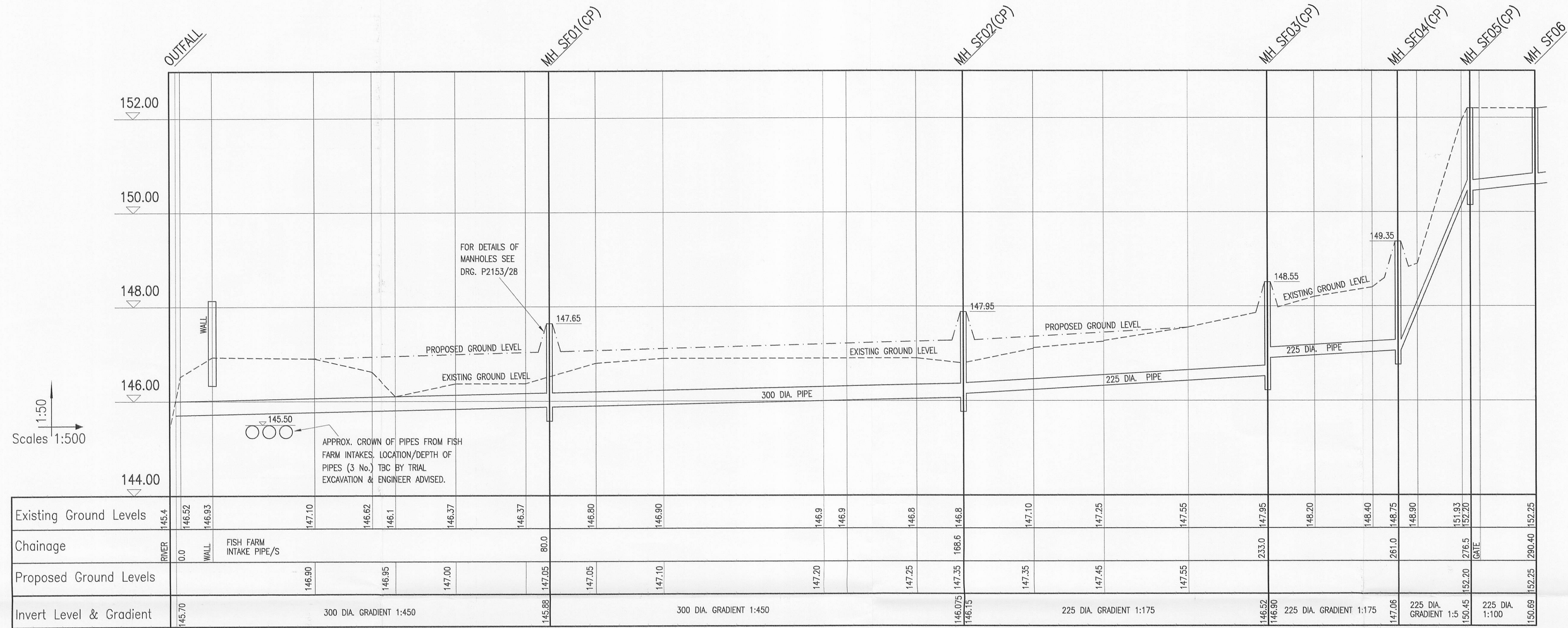
LONGITUDINAL SECTION OUTFALL TO MH SF06
