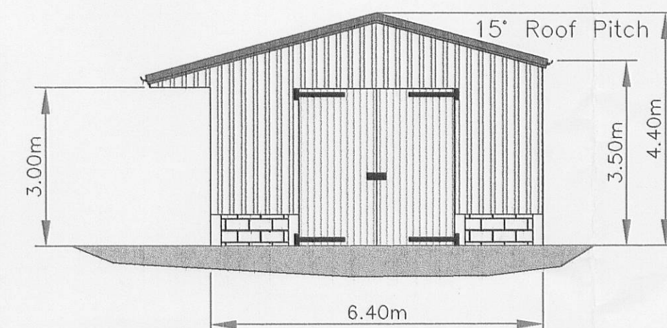
WEST FACING ELEVATION
