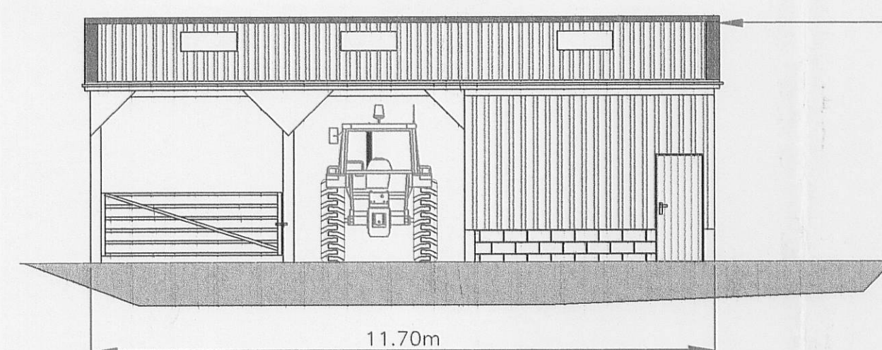
NORTH FACING ELEVATION
