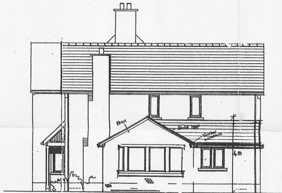
SIDE ELEVATION EXISTING (North east facing)
