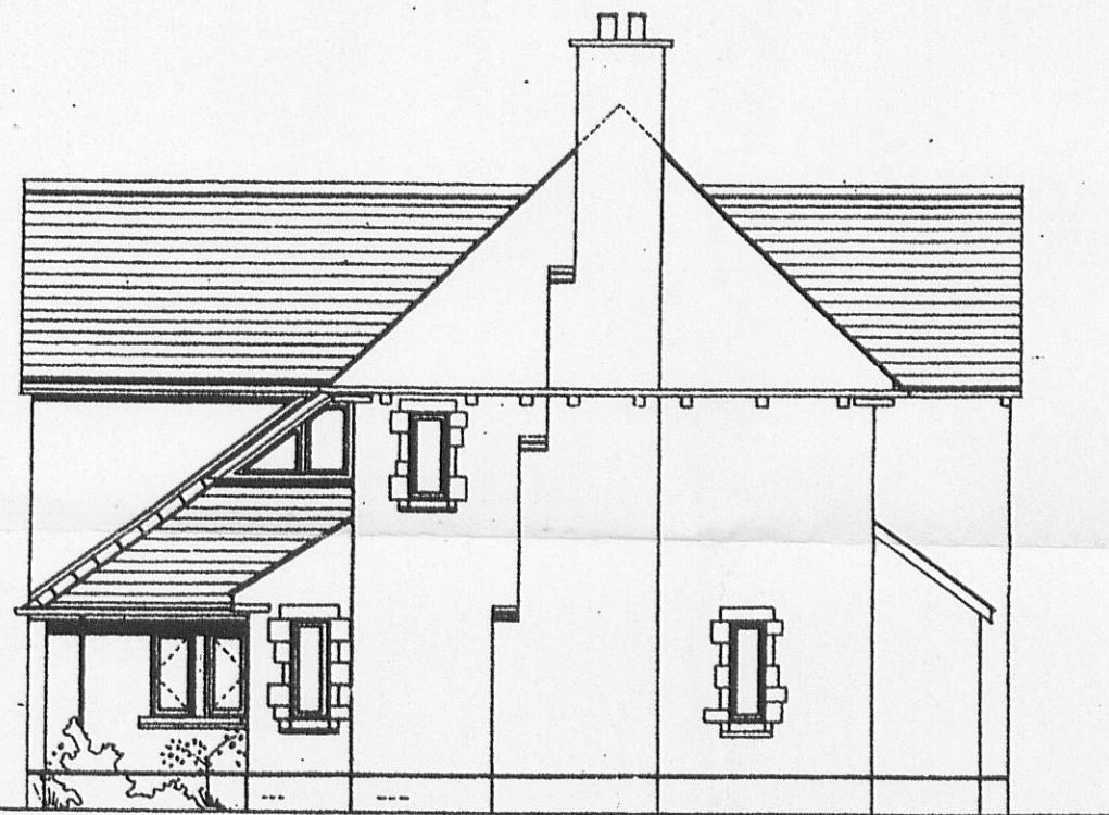
SIDE ELEVATION EXISTING (South west facing)
