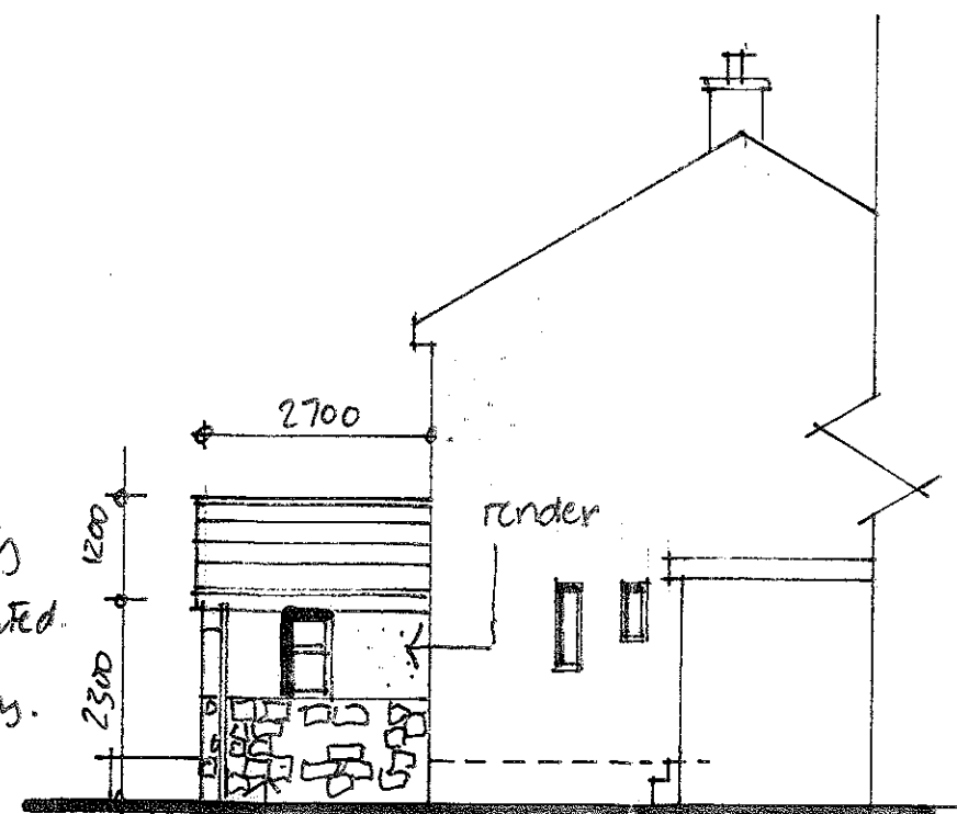
PROPOSED PART-SIDE ELEVATION.
