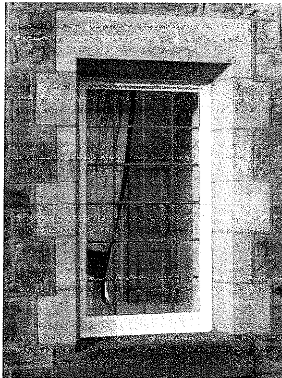
Pl. 3 Photograph showing an existing window surround and the detailing that would be repeated for new window openings.
