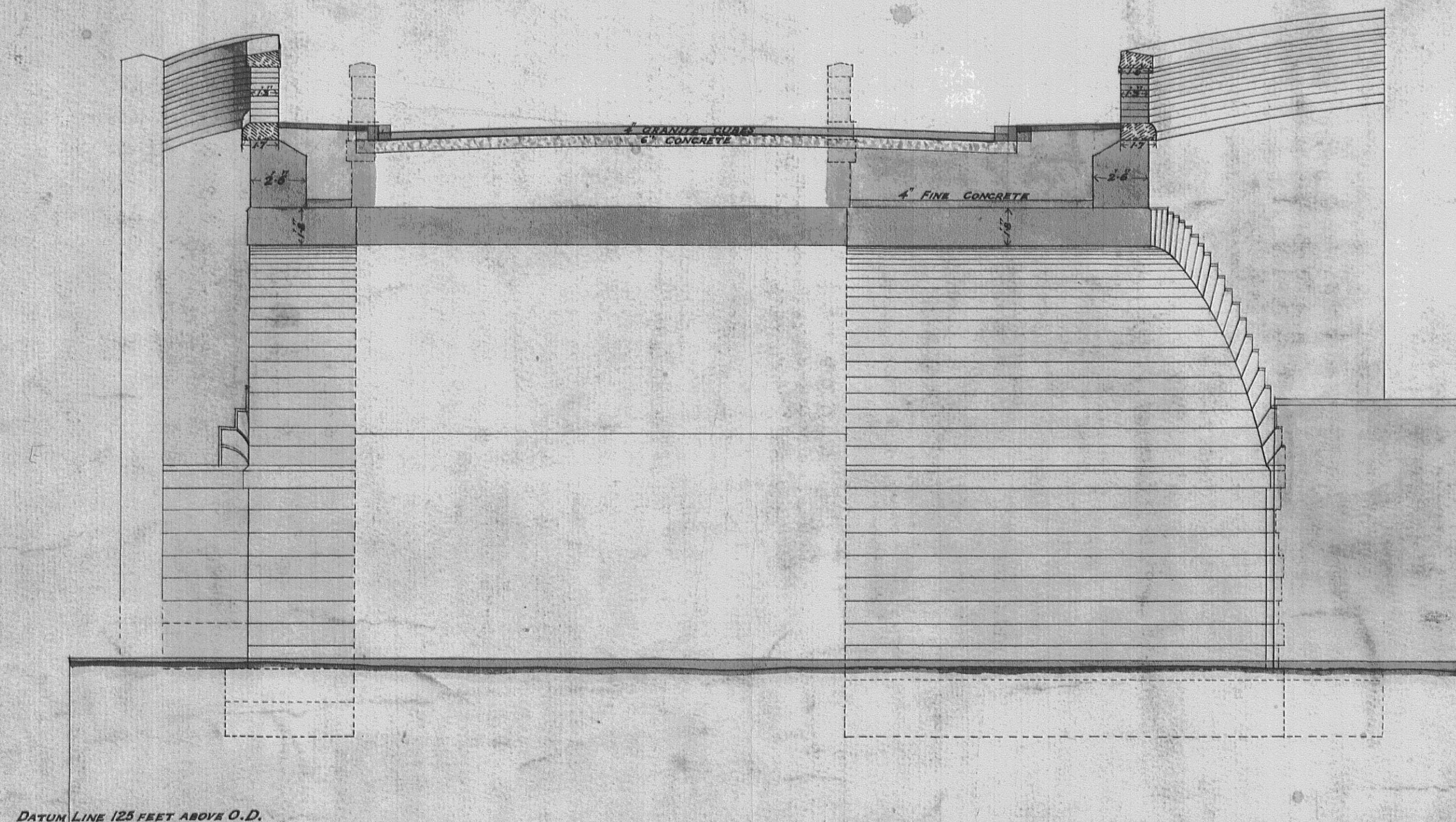
SECTION ON C.D.
