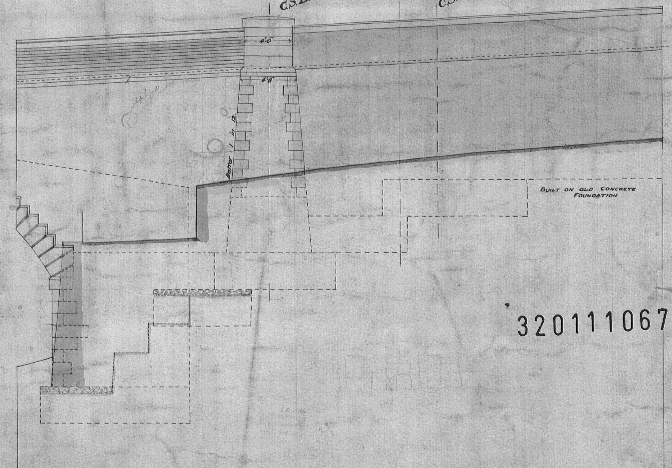
ELEVATION OF N.W. WING WALL
