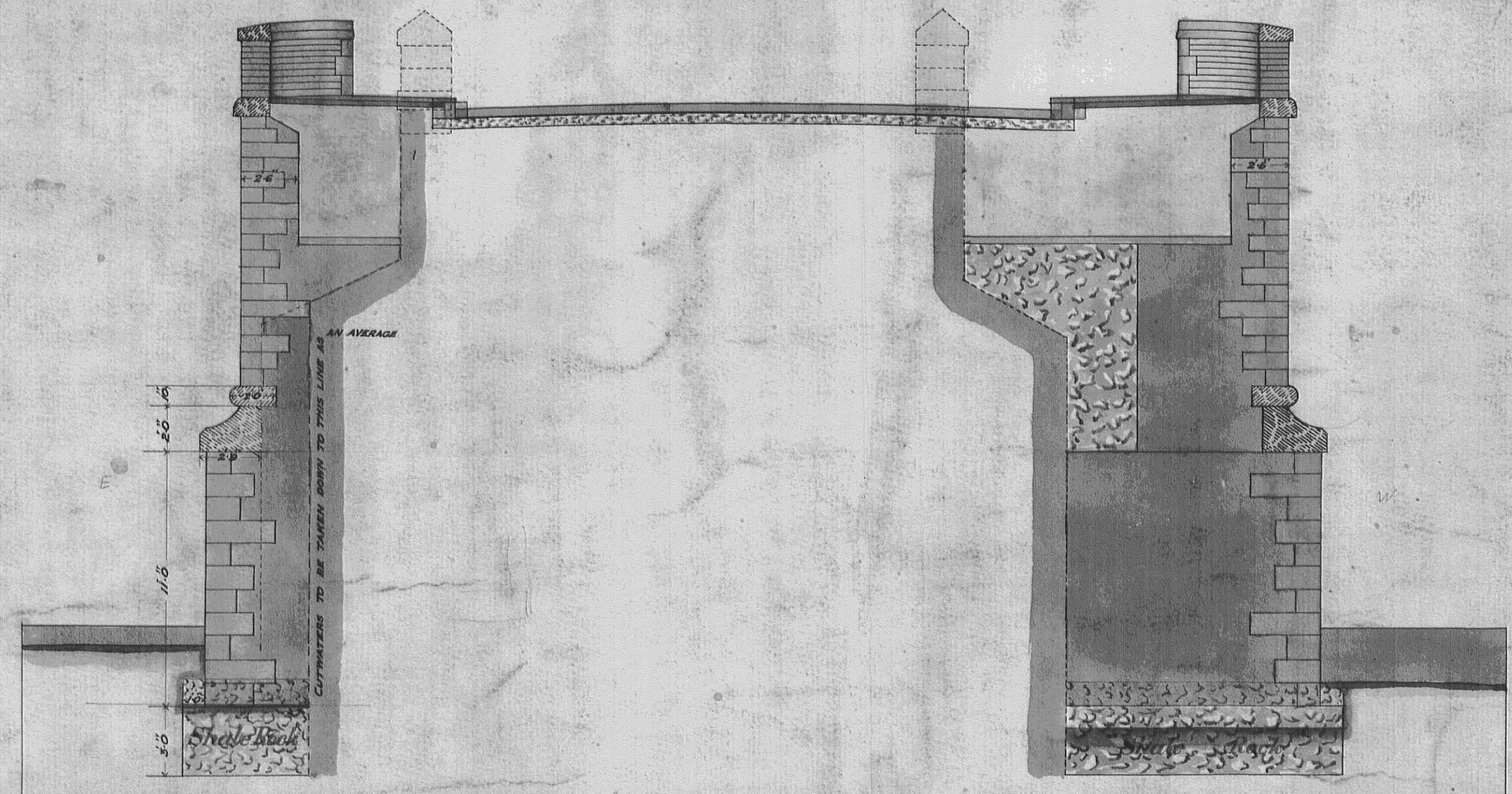
SECTION ON E.F. CS.LM.
