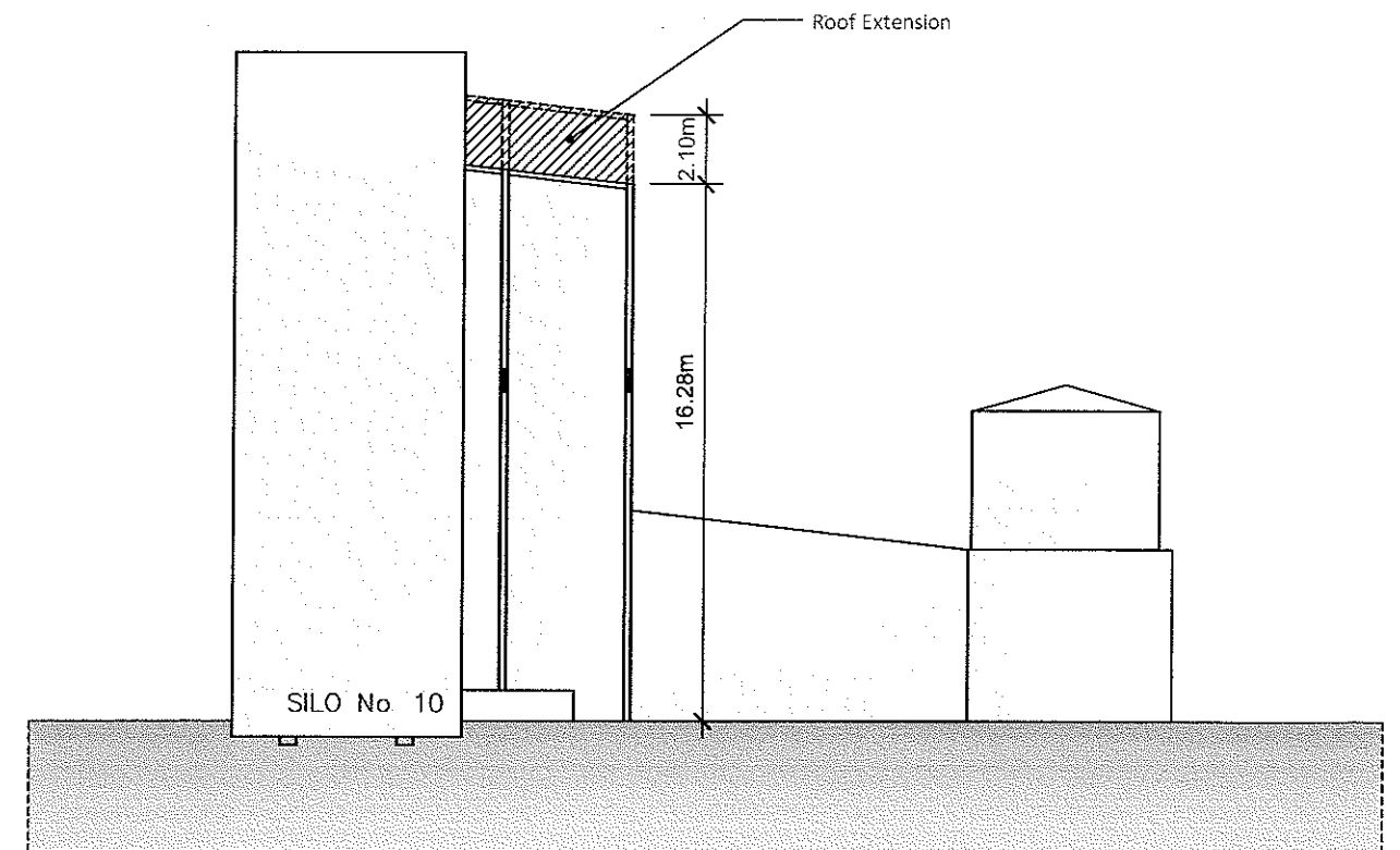
Proposed Elevation
