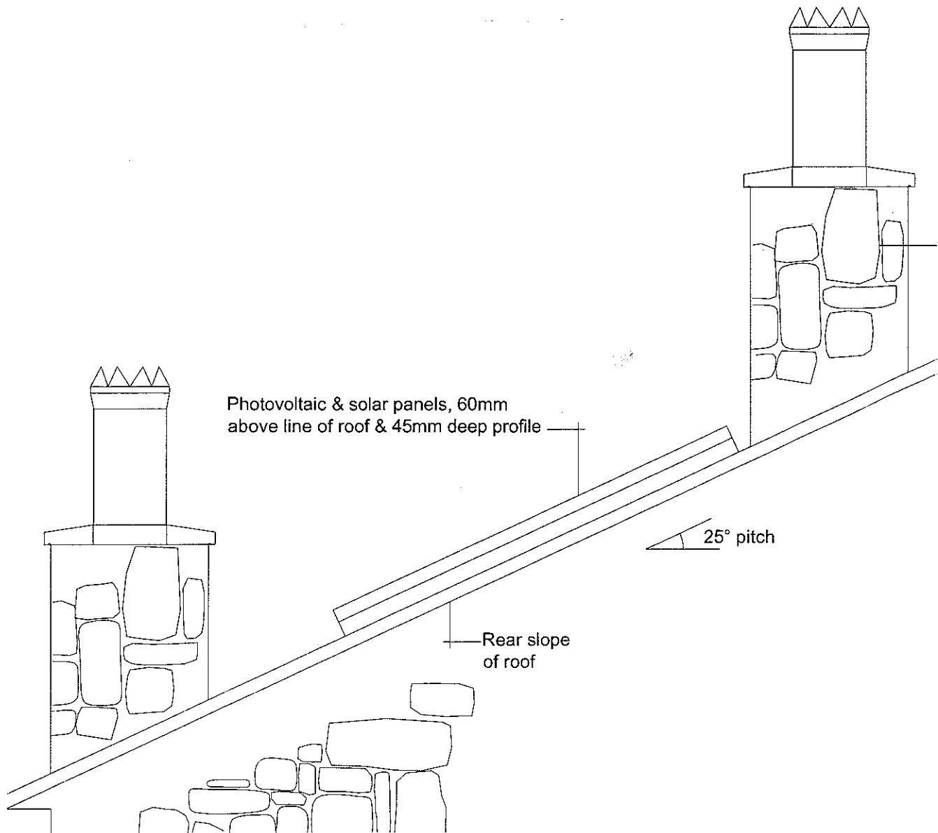
Solar PV panel detail 1:20
