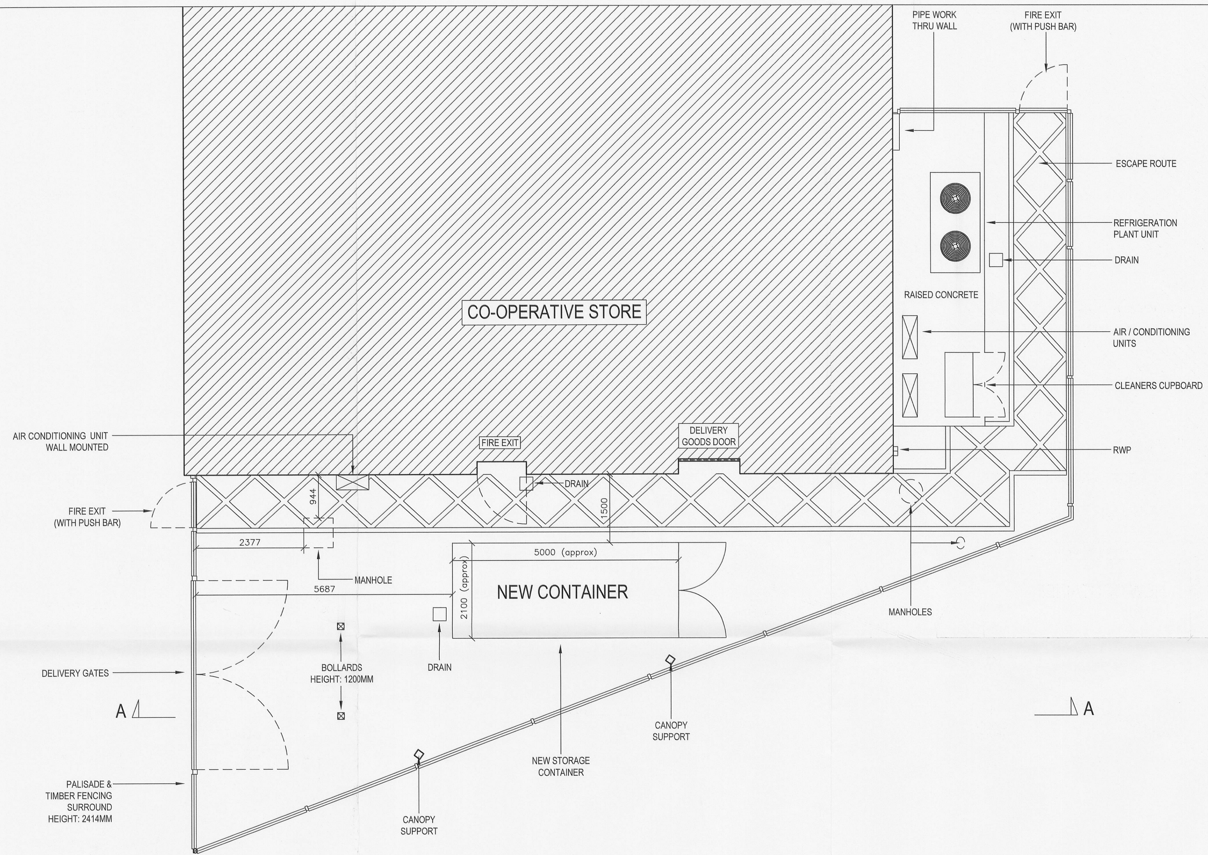
PROPOSED PLAN LAYOUT
