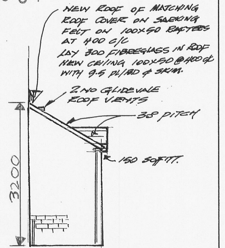
SIDE ELEVATION
