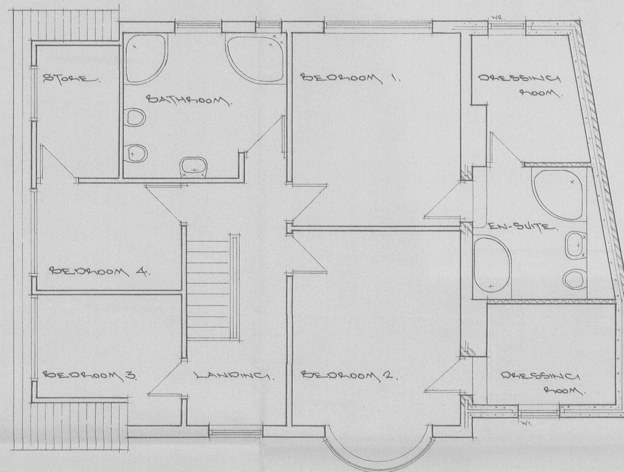
Proposed F. F. plan.
