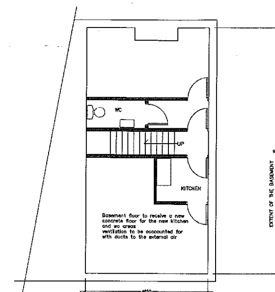
PROPOSED BASEMENT FLOOR PLAN
