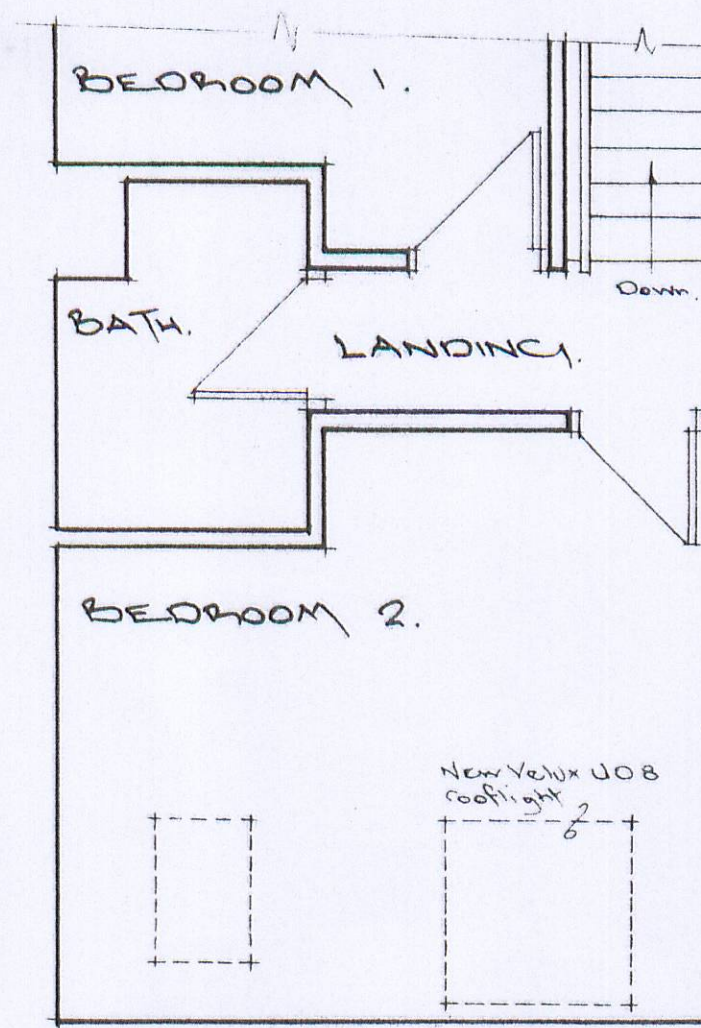
Proposed F. F. plan.
