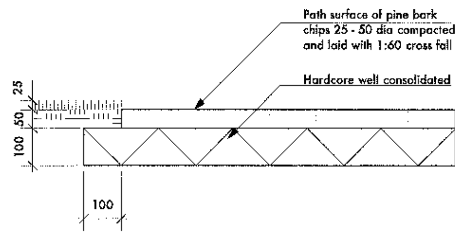
1 Pedestrian Path - pine bark Scale: 1:10
