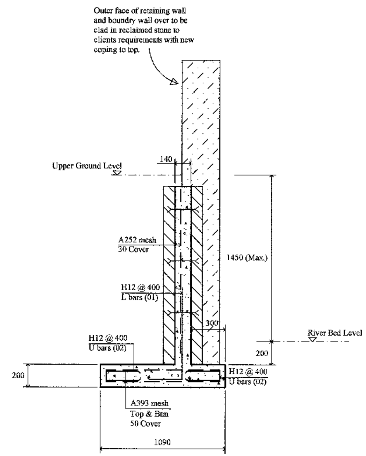
Typical Section
