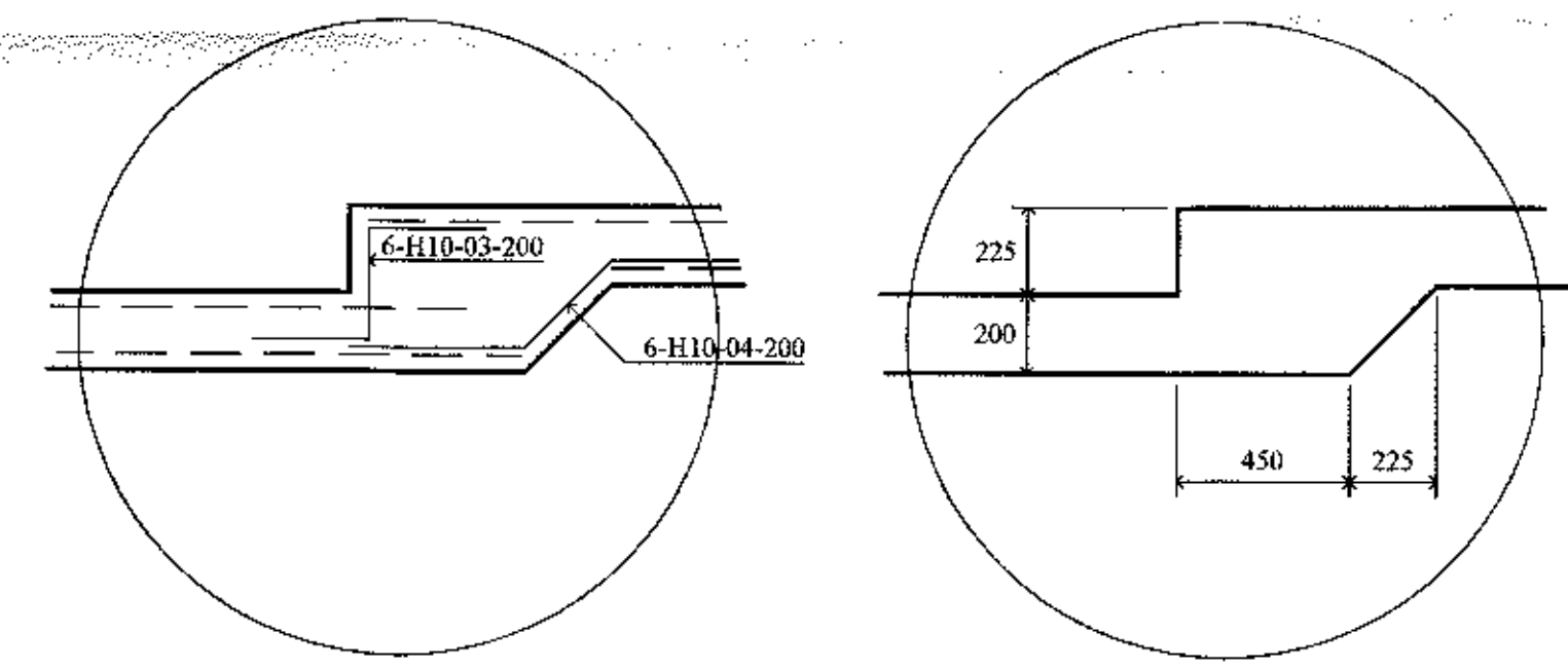
Typical Base Step Detail
