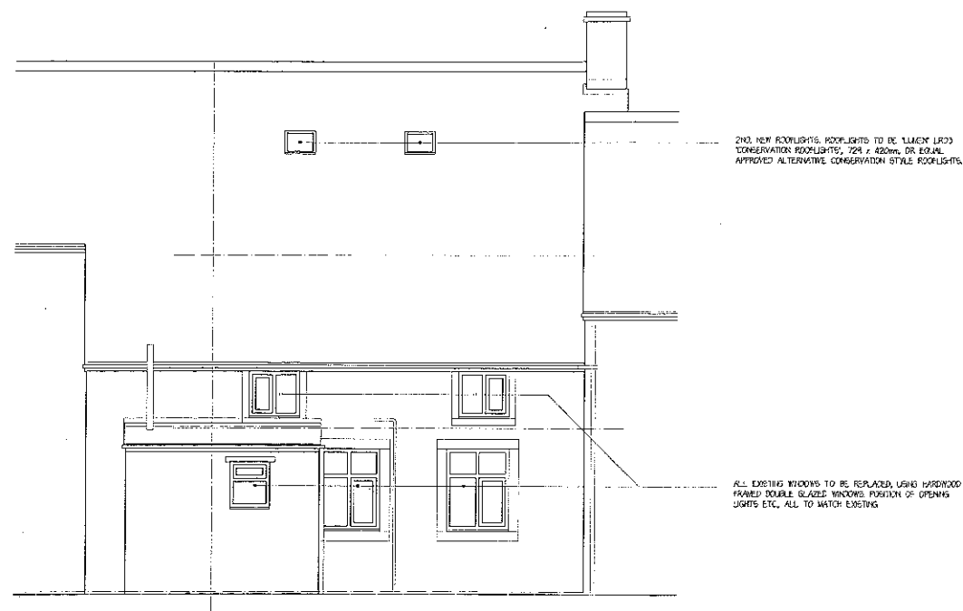
REAR ELEVATION
