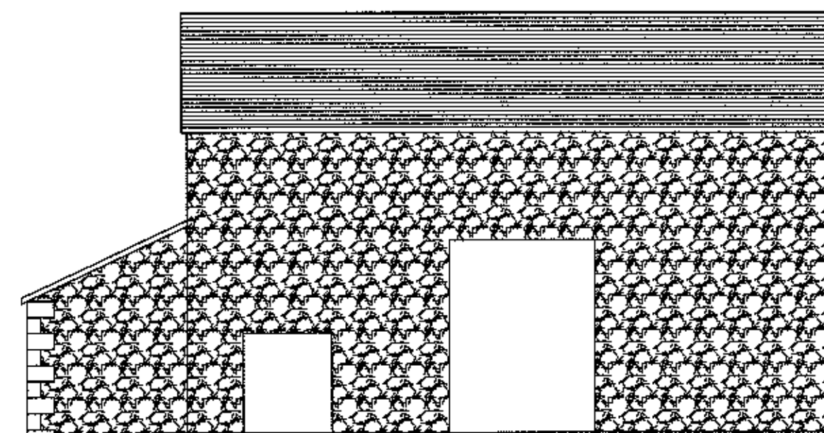
Existing Elevations North
