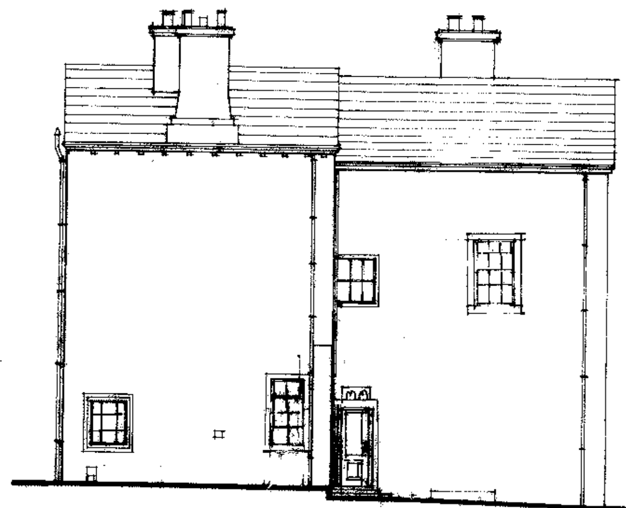
south elevation
