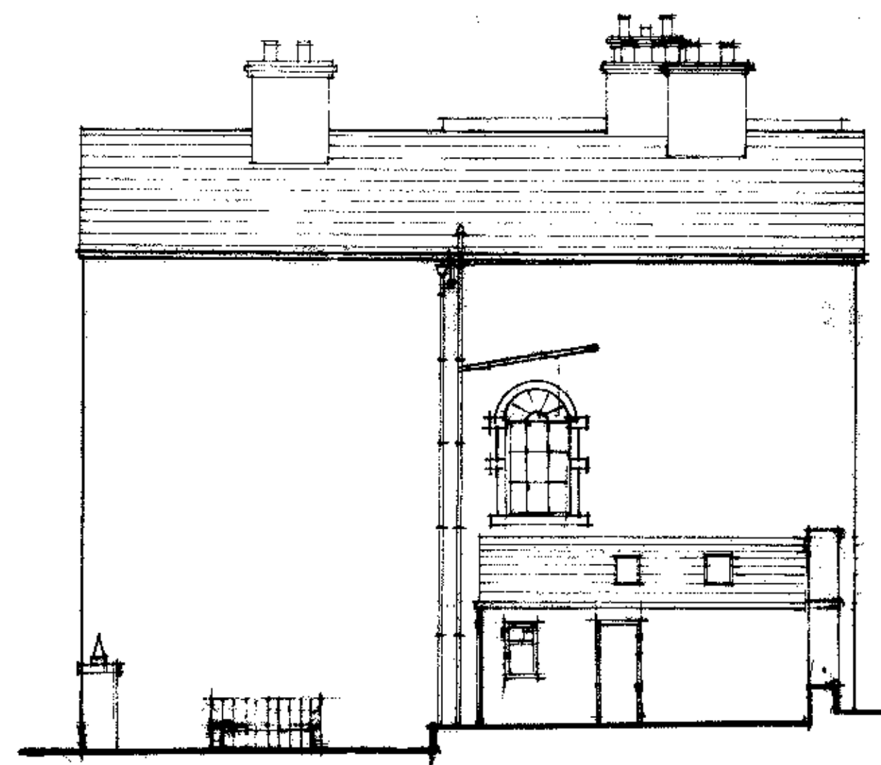
north elevation
