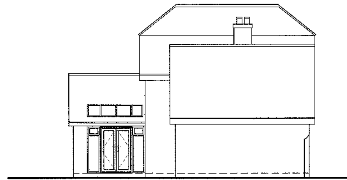
Existing Side (east) Elevation 1 : 100
