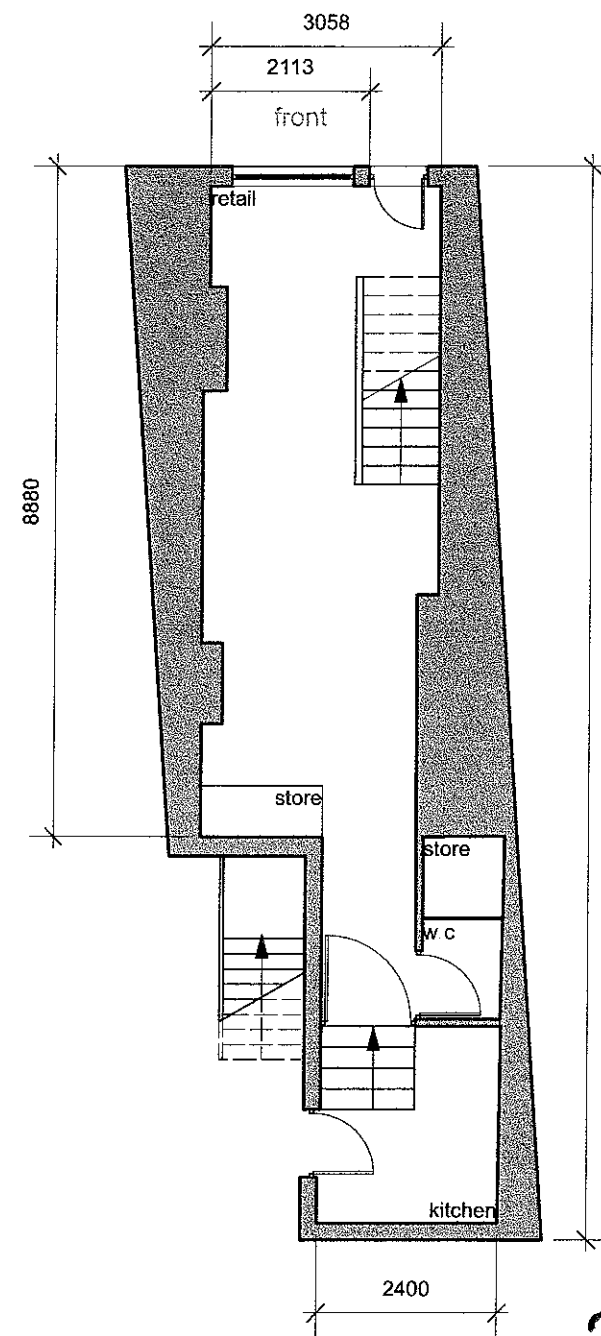
GROUND FLOOR
