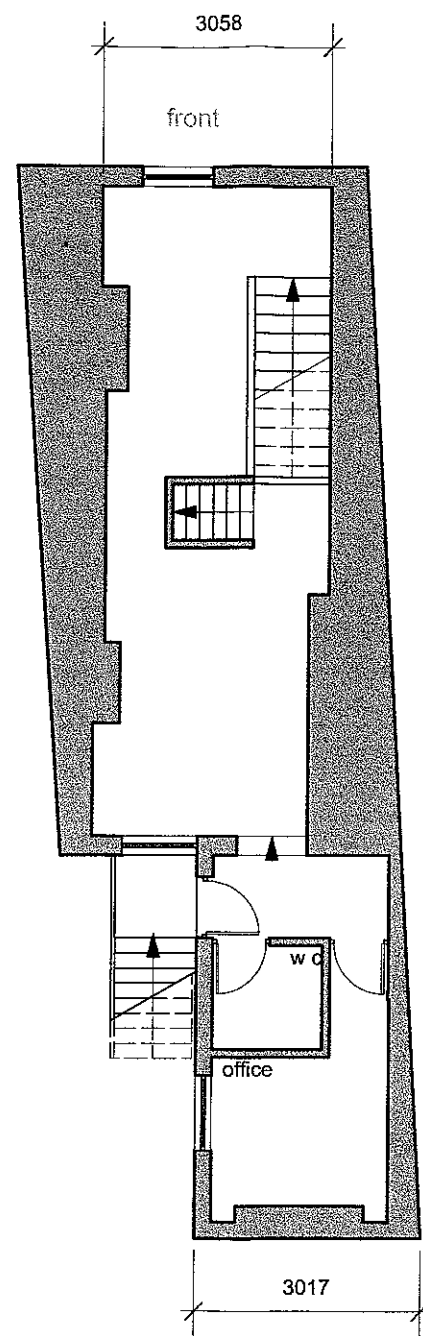
FIRST FLOOR
