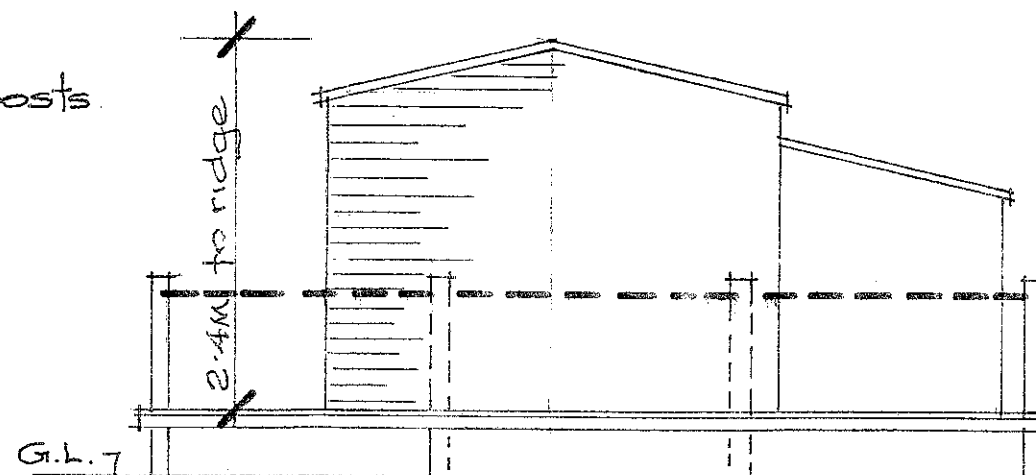
rear elevation 3.
