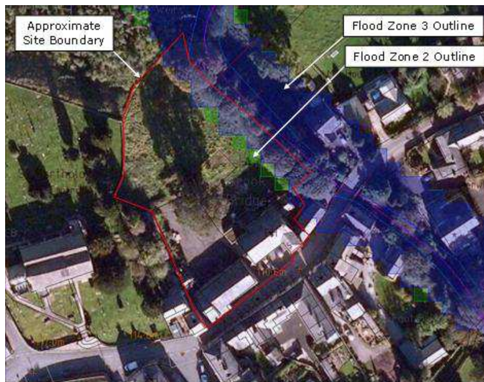
Figure 3: Zone 2 and 3 Flood Outlines
