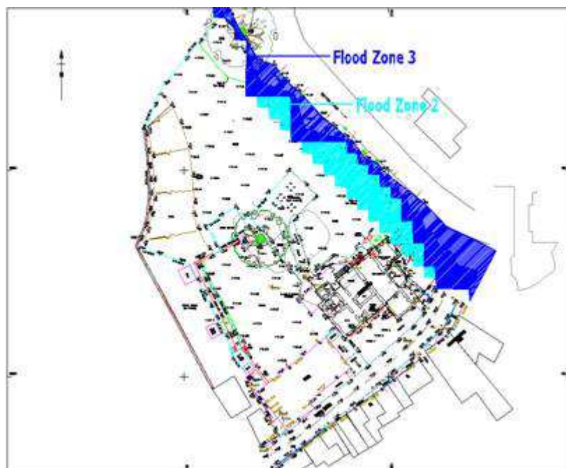
Figure 4: Detailed Site Flood Outlines
