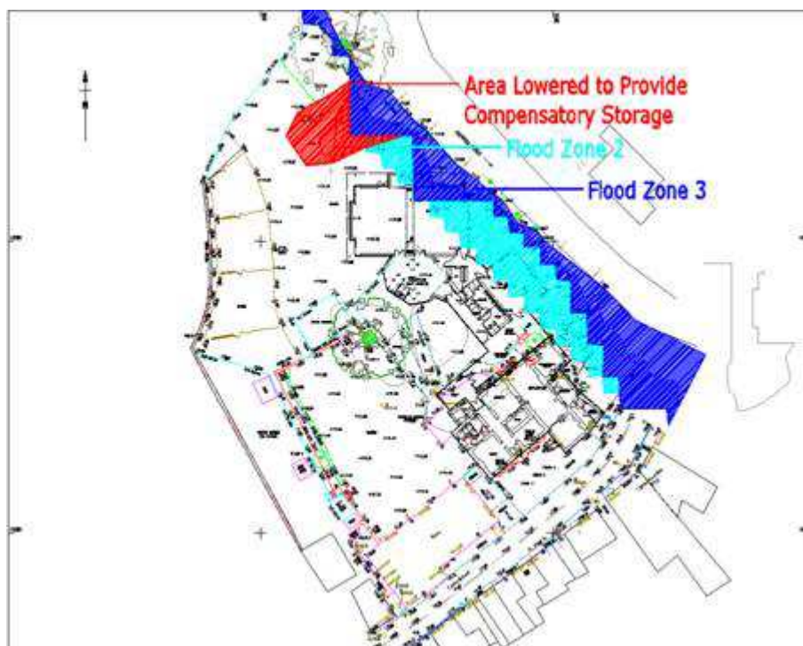
Figure 7: Potential Compensatory Flood Storage Area
