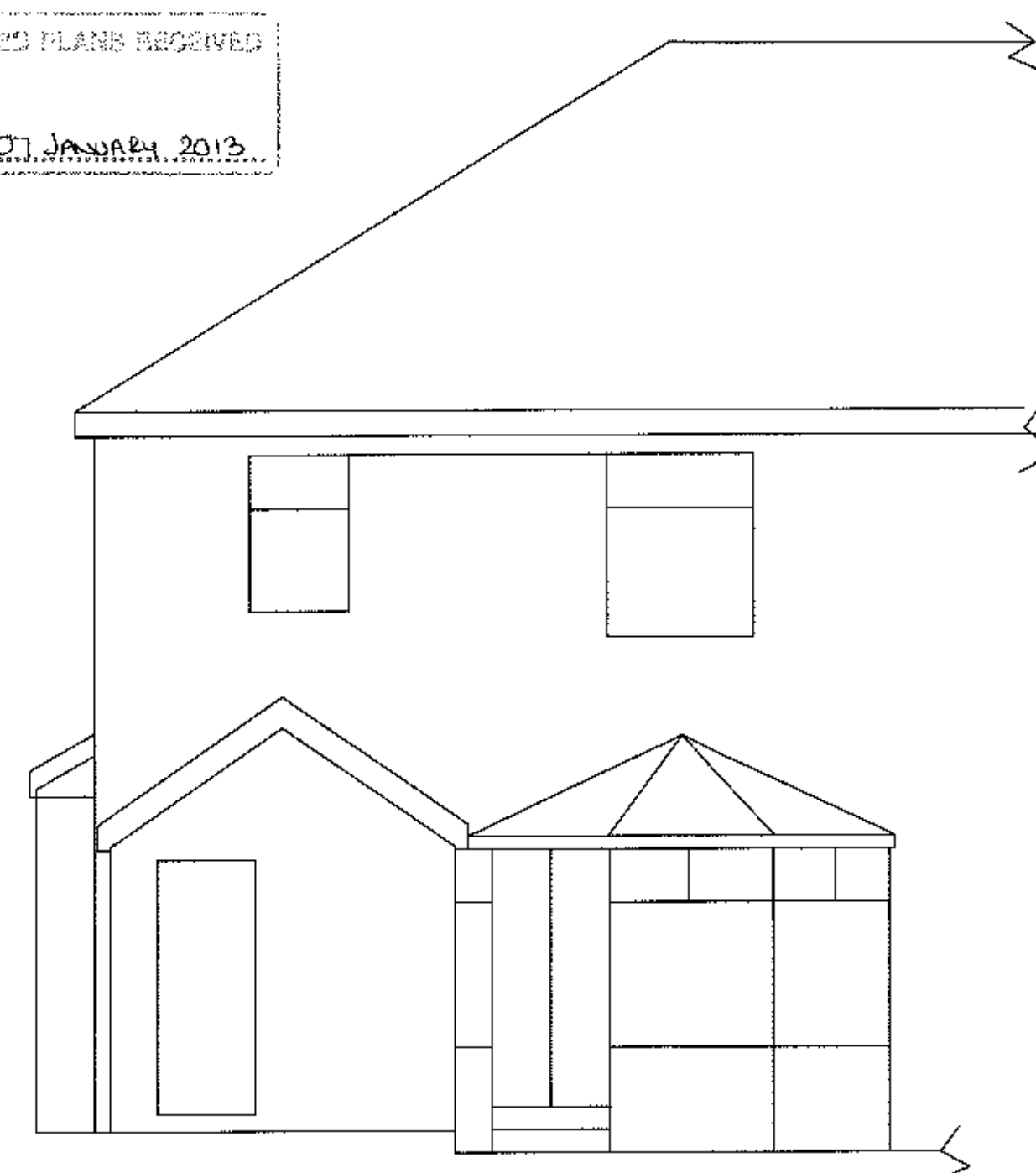
EXISTING REAR
