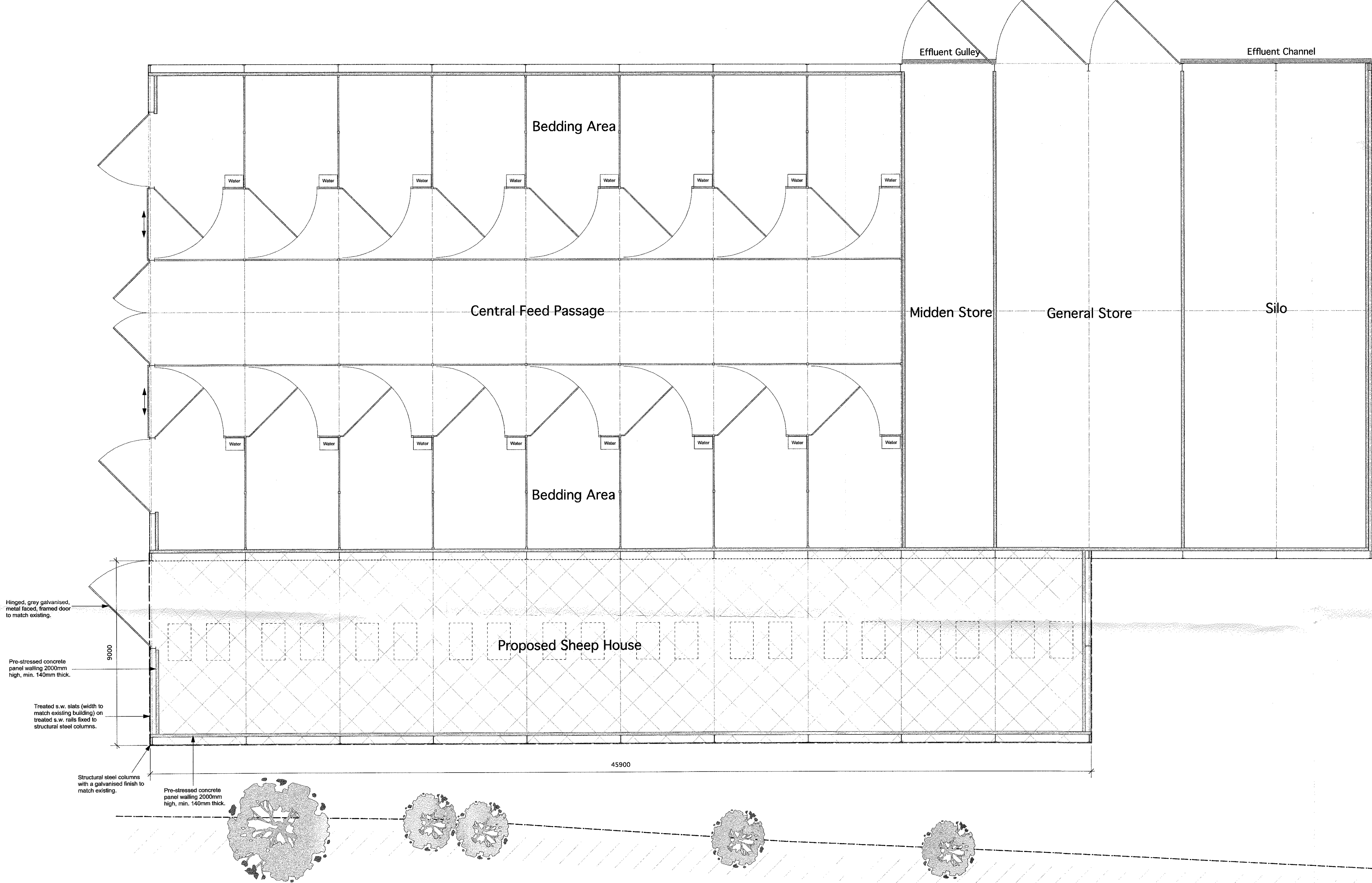
Existing and Proposed Plan
