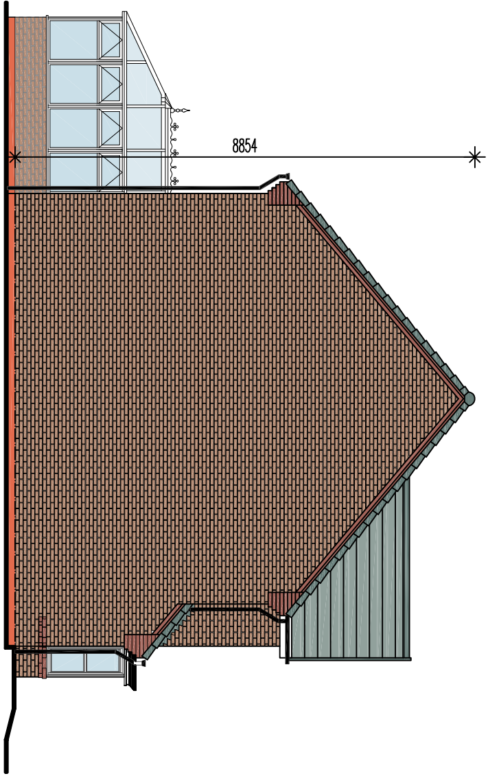
side elevation - with conservatory option
