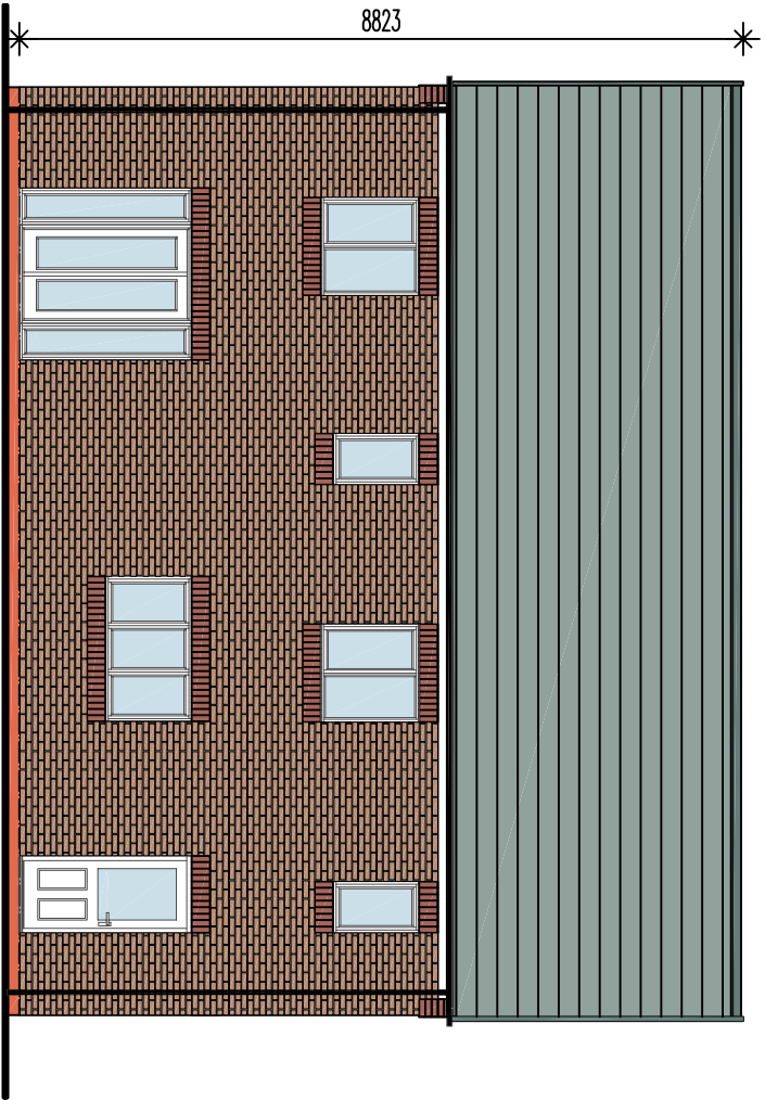
rear elevation
