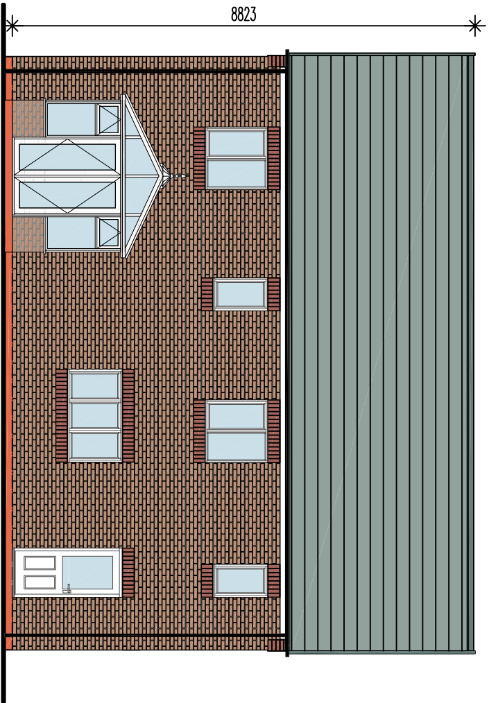
rear elevation - with conservatory option
